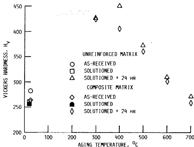
Figure 7.—Vickers hardness for unreinforced matrix and composite matrix in both solutioned and aged conditions (Vickers hardness indentions made at 200-g load).
