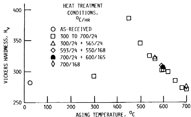
Figure 6.—Vickers hardness as function of aging condition for unreinforced matrix (Vickers hardness indentions made at 200-g load).
