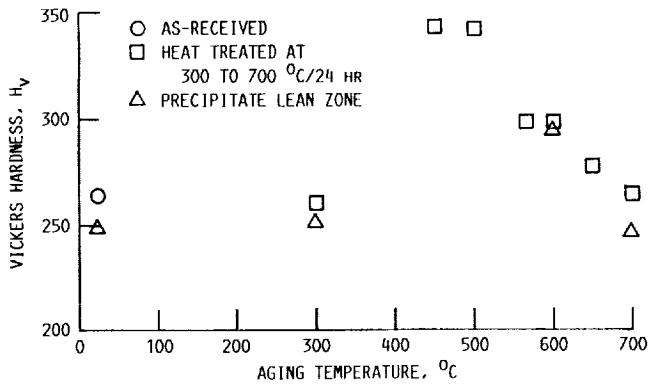
Figure 8.—Aging response of Vickers hardness for composite matrix (hardness of precipitate lean zone also included; Vickers hardness indentations made at 200-g load).
