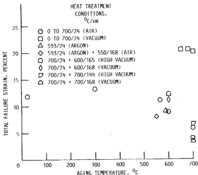
Figure 13.—Room-temperature failure strain as function of aging for unreinforced matrix.
