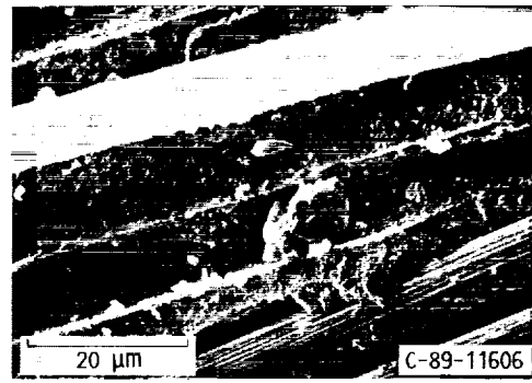
FIGURE 8. - CLEAVED SURFACE OF T-40R UNIDIRECTIONAL COMPOSITE SHOWING INTERFACIAL FAILURE.
