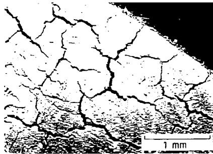
(b) CELION 6000/PMR-15 COMPOSITE AFTER 1212 HR OF AGING. CRACKS RUN PARALLEL TO FIBERS.
