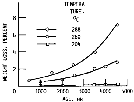
FIGURE 3. - AIR-AGING OF CELION 6000/PMR-15 UNIDIRECTIONAL COMPOSITES.
