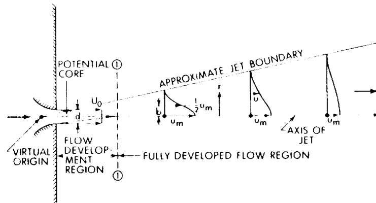
Figure 6. Definition sketch of circular turbulent jets.
