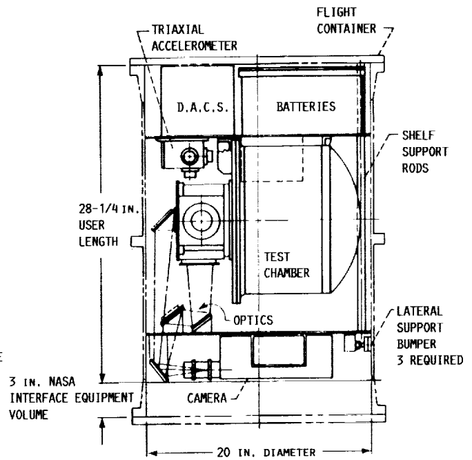
SET-UP OF EXPERIMENT IN CONTAINER.
