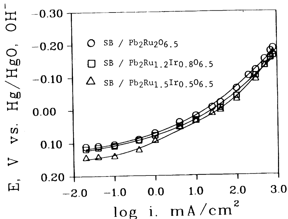
Fig. 3. Tafel plot for O 2 reduction on Pb 2 Ru 2 O 6.5 (thin porous coating) in O 2 -saturated 1 M KOH. The current values (in mA) for 2500 rpm from Fig. 2 were corrected for mass transport using I L = 1.75 mA.
