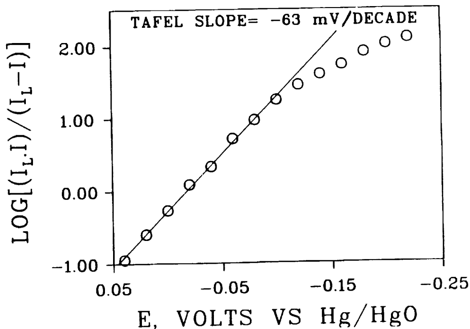
Fig. 3. Tafel plot for O 2 reduction on Pb 2 Ru 2 O 6.5 (thin porous coating) in O 2 -saturated 1 M KOH. The current values (in mA) for 2500 rpm from Fig. 2 were corrected for mass transport using I L = 1.75 mA.
