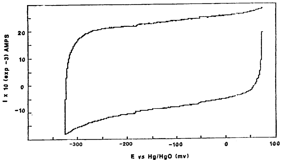
FIG. 9 CYCLIC VOLTAMMOGRAM
