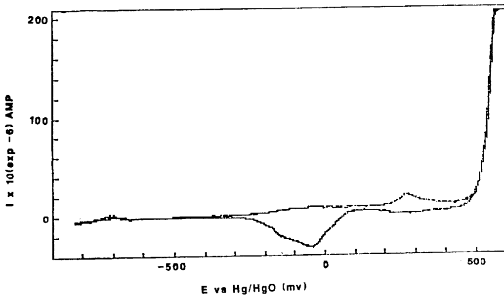
Sweep: 600 to -826 mv, 1 mv/s, 80 deg. C, Nitrogen, 30%KOH FIG. 5 CYCLIC VOLTAMMOGRAM; GOLD WIRE SCREEN
