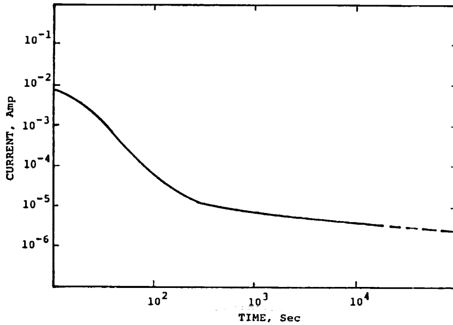
FIG. 3. CORROSION CURRENT
