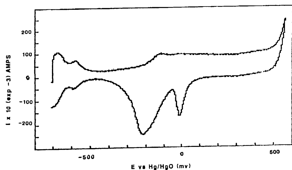
Sweep: 564 to -706 mv, 1 mv/s, 24 deg.C, Nitrogen, 30%KOH FIG. 6 CYCLIC VOLTAMMOGRAM
