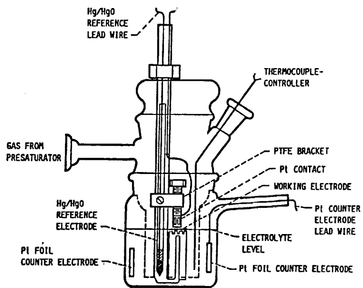
FIG. 1. FLOATING HALF-CELL
