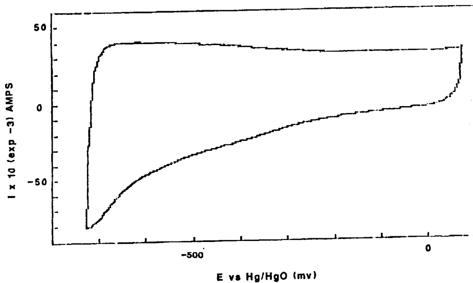
FIG. 10 CYCLIC VOLTAMMOGRAM
