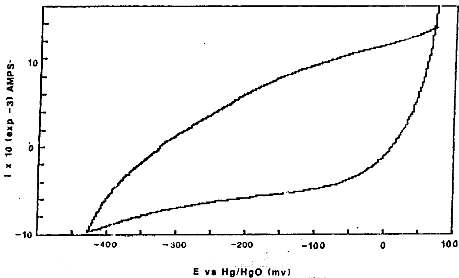
FIG. 11 CYCLIC VOLTAMMOGRAM
