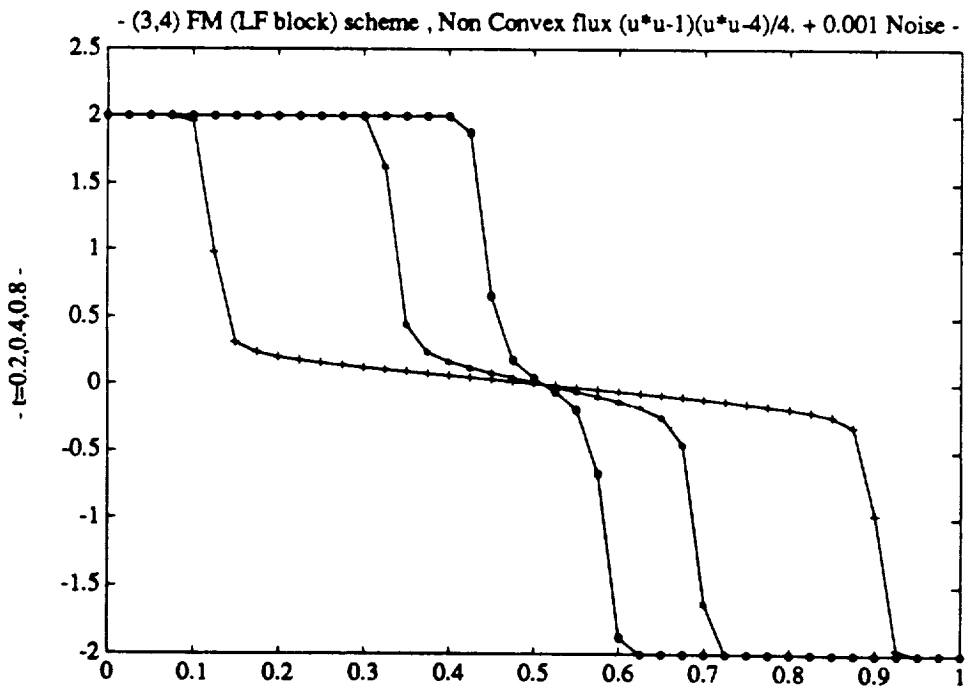
- Solution wave - Figure 3.7.4 -
