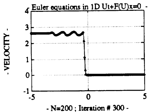
- (3,6) FM scheme , figure 5.4.2 -
