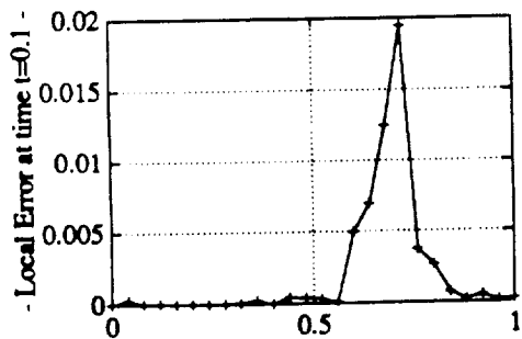
- (3,4) CD scheme + uniform ENO-Roe-4 filter -
