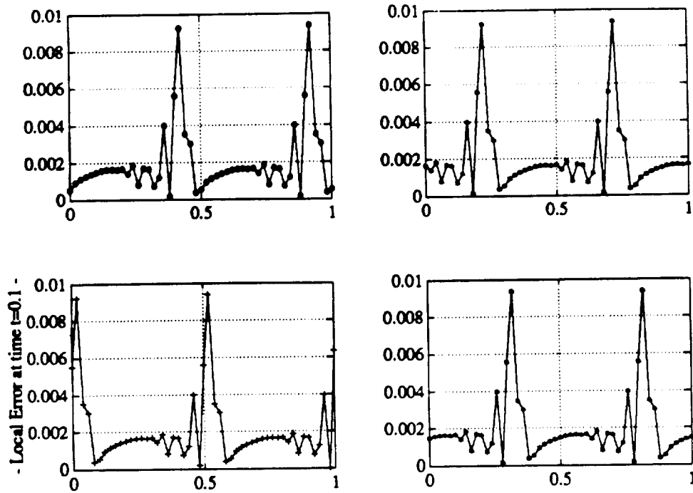
- (3,2) CD scheme + uniform ENO-Roe-2 filter , figure 2.1 -
