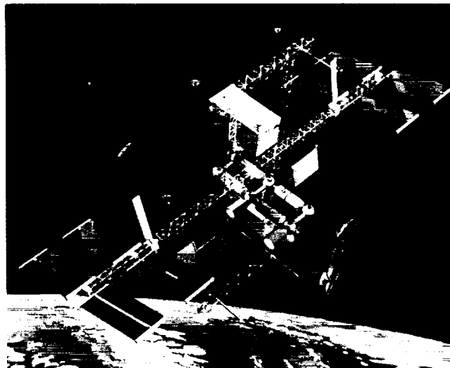
"DUAL KEEL" — this picture illustrates an artist's conception of a more recent Space Station configuration, known as the "dual keel." In comparison to the "power tower" this configuration offers a number of advantages. The laboratory and habitat modules have been moved closer to the center of gravity, more space is provided for attached payloads and greater structural stiffness is realized.
