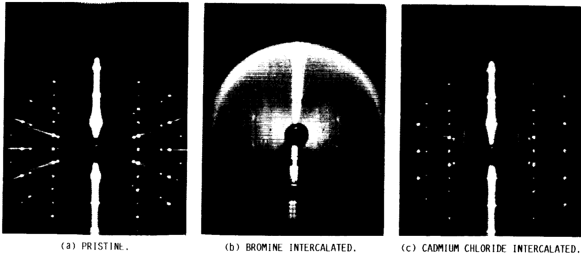
FIGURE 1. - X-RAY DIFFRACTION HOL PRECESSION PHOTOGRAPHS OF HOPG.
