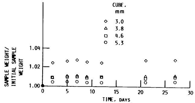
FIGURE 4. - DEGRADATION OF VARIOUS SIZE SAMPLES OF CADMIUM CHLORIDE INTERCALATED HOPG OVER TIME.
