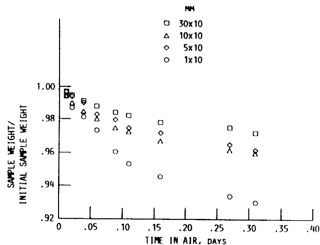
FIGURE 3. - WEIGHT LOSS OF VARIOUS SIZE SAMPLES OF SAMPLES OF BROMINE INTERCALATED HOPG OVER TIME.
