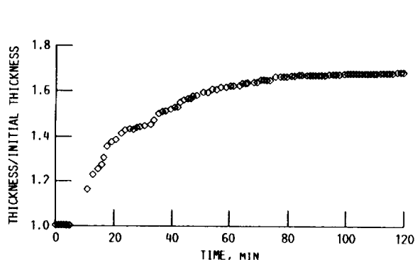
FIGURE 2. - EXPANSION IN THE CRYSTALLOGRAPHIC "C" DIRECTION OF HOPG UPON EXPOSURE TO 165 TORR OF BROMINE VAPOR.
