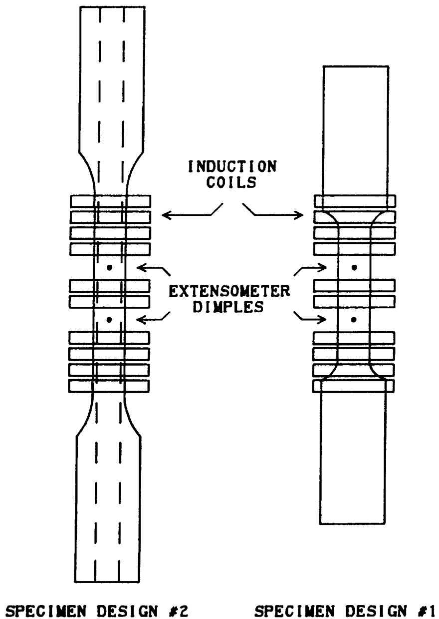
Figure 3.4 - Location of Induction Heater Coils
