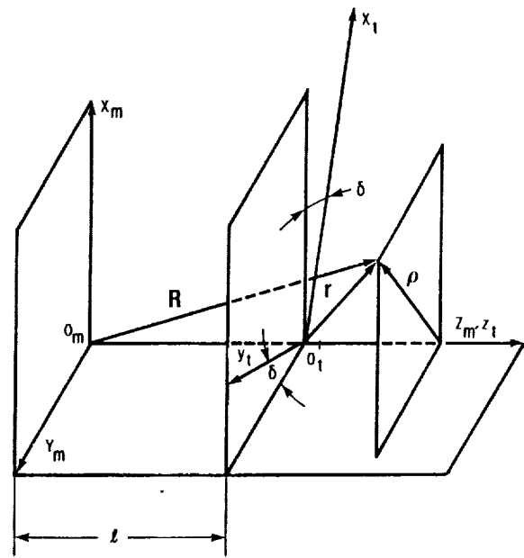
FIGURE 2. - COORDINATE TRANSFORMATION.
