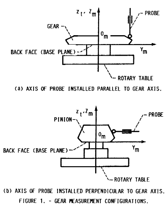
FIGURE 1. - GEAR MEASUREMENT CONFIGURATIONS.
