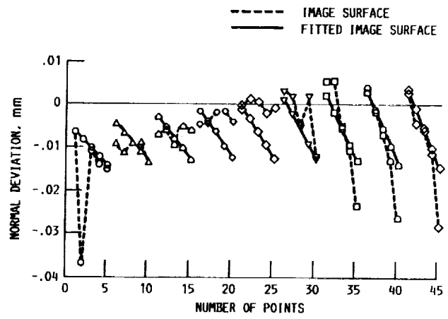
FIGURE 8. - PLOT OF DEVIATIONS OF IMAGE SURFACE \Sigma_r^* AND FITTED IMAGE SURFACE \Sigma_t^* .
