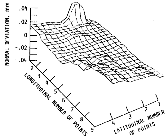
FIGURE 5. - DEVIATION OF REAL SURFACE \Sigma_r .
