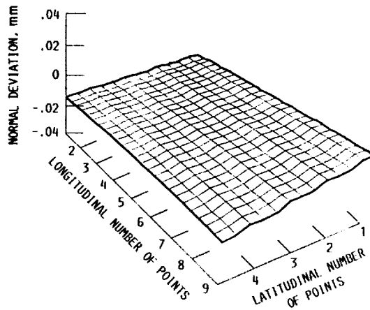
FIGURE 9. - DEVIATION OF FITTED IMAGE SURFACE \Sigma_t^* .
