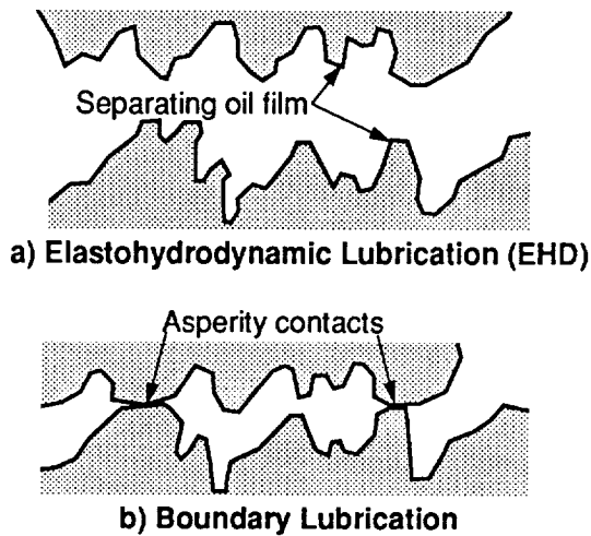
FIGURE 6. LUBRICATION REGIMES
