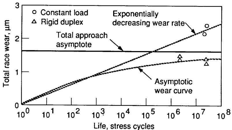
FIGURE 14. BALL BEARING DATA POINTS Chemical Wear: Preload Loss Bray-815Z, Foam/Phenolic, AISI 440C
