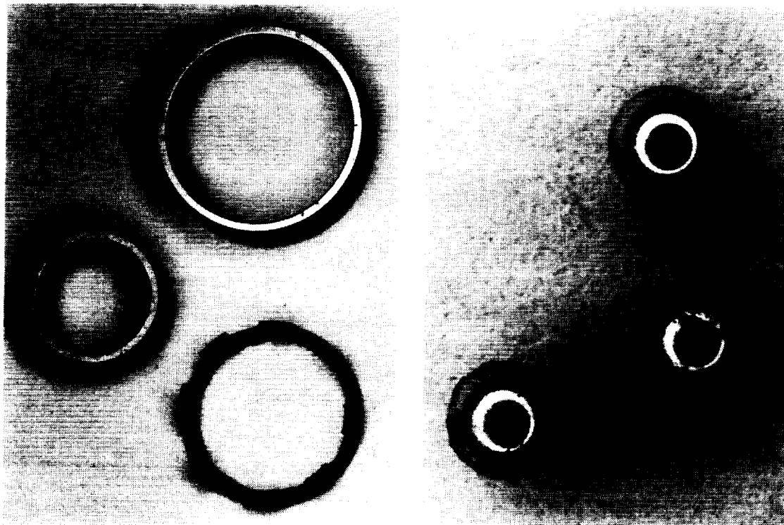
FIGURE 13a. RACES AND RETAINER FOLLOWING TEST
