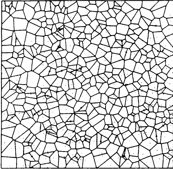
Primary tessellation #500
