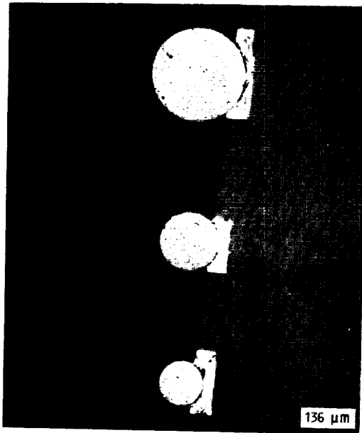
FIGURE 3. - SPREADING FROM PARTIALLY CAPPED CONTACTS.
