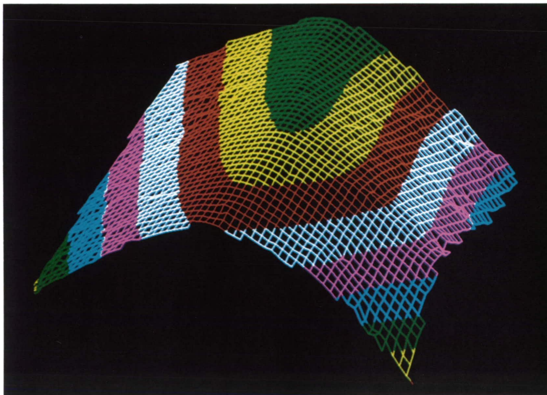
Figure 12. Three-dimensional perspective of region near Crete Station. Area shown in figure corresponds to Map 16. Bands change color every 50 meters of elevation. View is from SSE.
