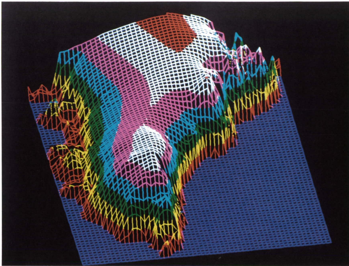
Figure 11. Three-dimensional perspective of Greenland (south of 72° N) from grid elevations. Bands change color every 500 meters of elevation. View is from SSW.
