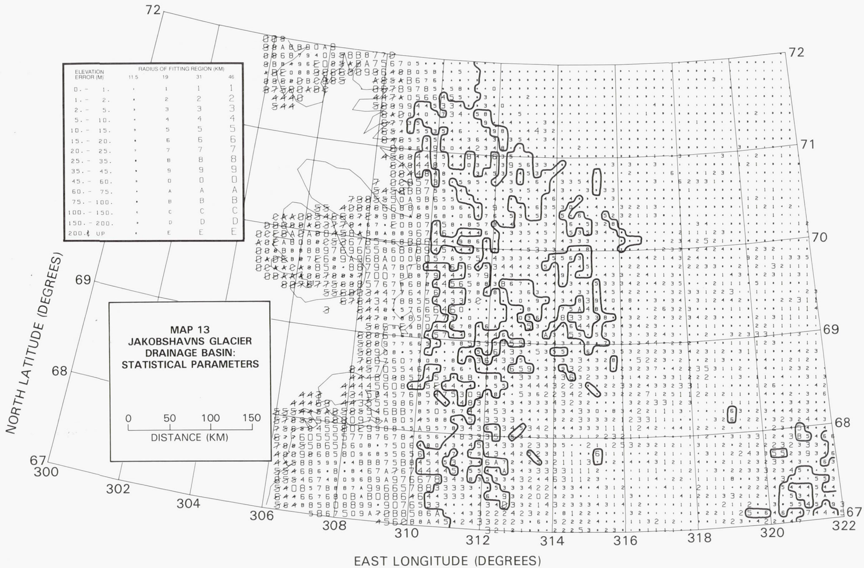
Map 13. Statistical parameters of grid elevations calculated in Jakobshavns Glacier region (Map 12). Physical size of number or letter at each gridpoint indicates size of gridding region at that gridpoint. Numerical size or alphabetical order indicates magnitude of elevation error (one standard deviation) at each gridpoint. Inset table provides key to sizes of fitting regions and magnitudes of elevation errors. Solid line encloses extended areas where derived elevation error exceeds \pm 10 meters.
