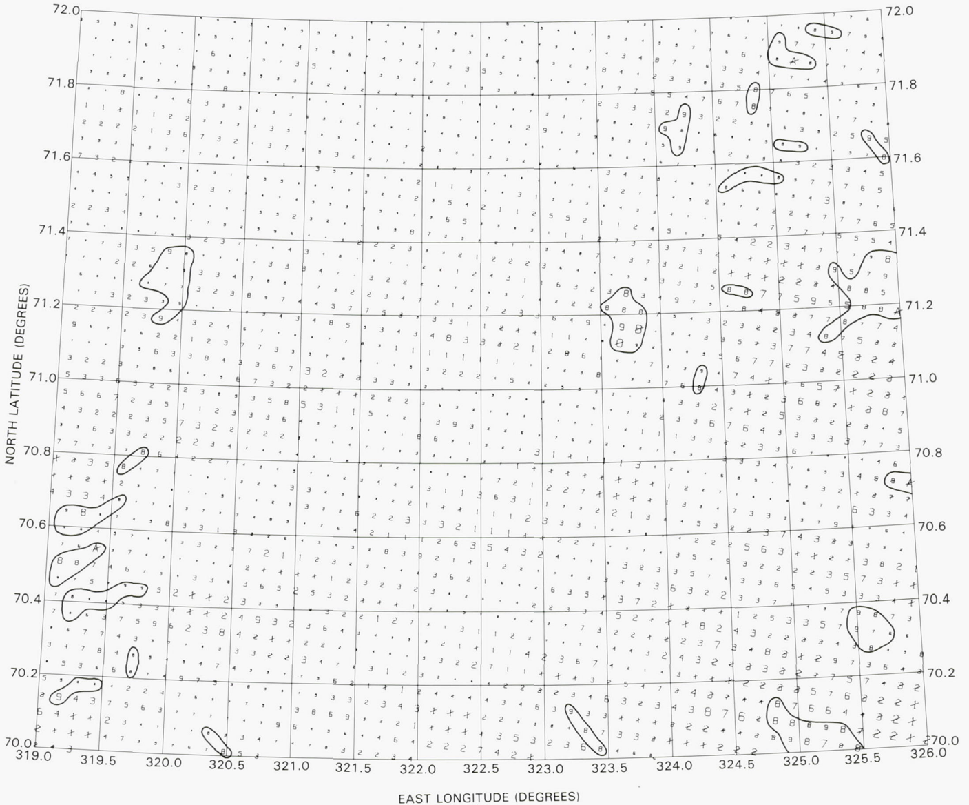
MAP 15 CRETE STATION REGION: STATISTICAL PARAMETERS 0 20 40 60 80 100 ─────────── DISTANCE (KM)
