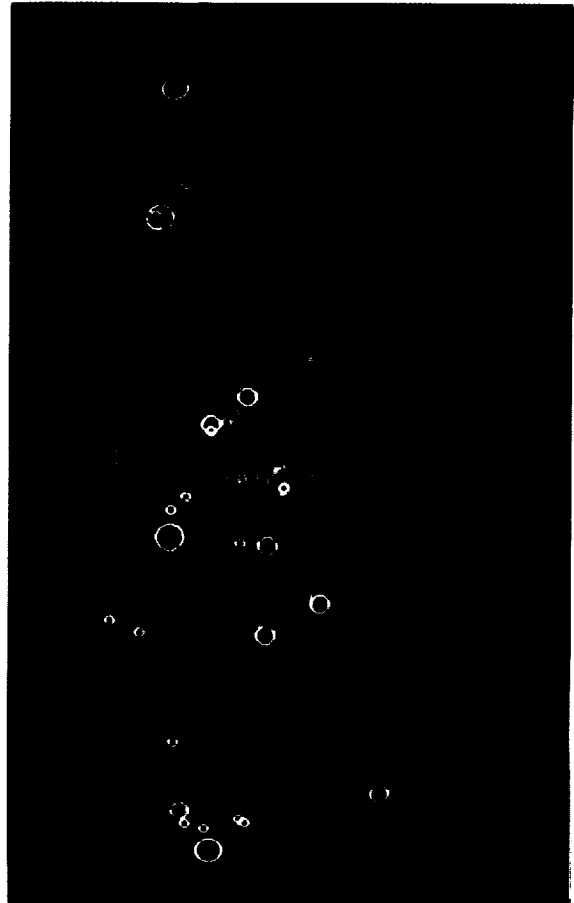
Figure 3. Same as Figure 2, but showing in white the Abell clusters which are not within a supercluster (more than 25 Mpc from all other clusters).
