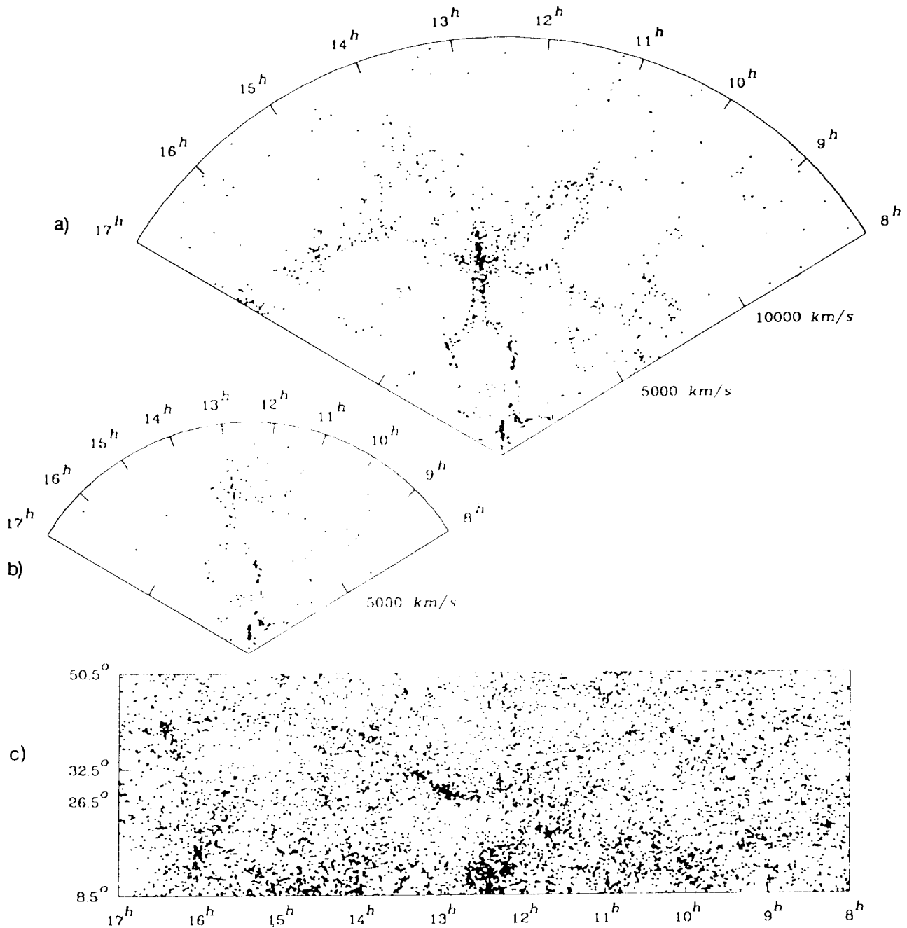
Figure 5 (from de Lapparent et al., 1986) - (a) Map of observed velocity plotted vs. right ascension in the declination wedge 26.5^\circ - 32.5^\circ , for 1061 objects with m_B \leq 15.5 and velocity \leq 15,000 \text{ km s}^{-1} . (b) same as (a), but for 182 galaxies with m_B \leq 14.5 and velocity \leq 10,000 \text{ km s}^{-1} . (c) Projected map of 7031 objects with m_B \leq 15.5 .
