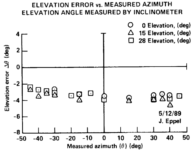
Figure 16. Elevation error versus measured azimuth (lab results).
