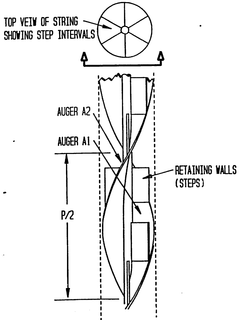
FIGURE 1. VIEWS OF THE DRILL STRING
