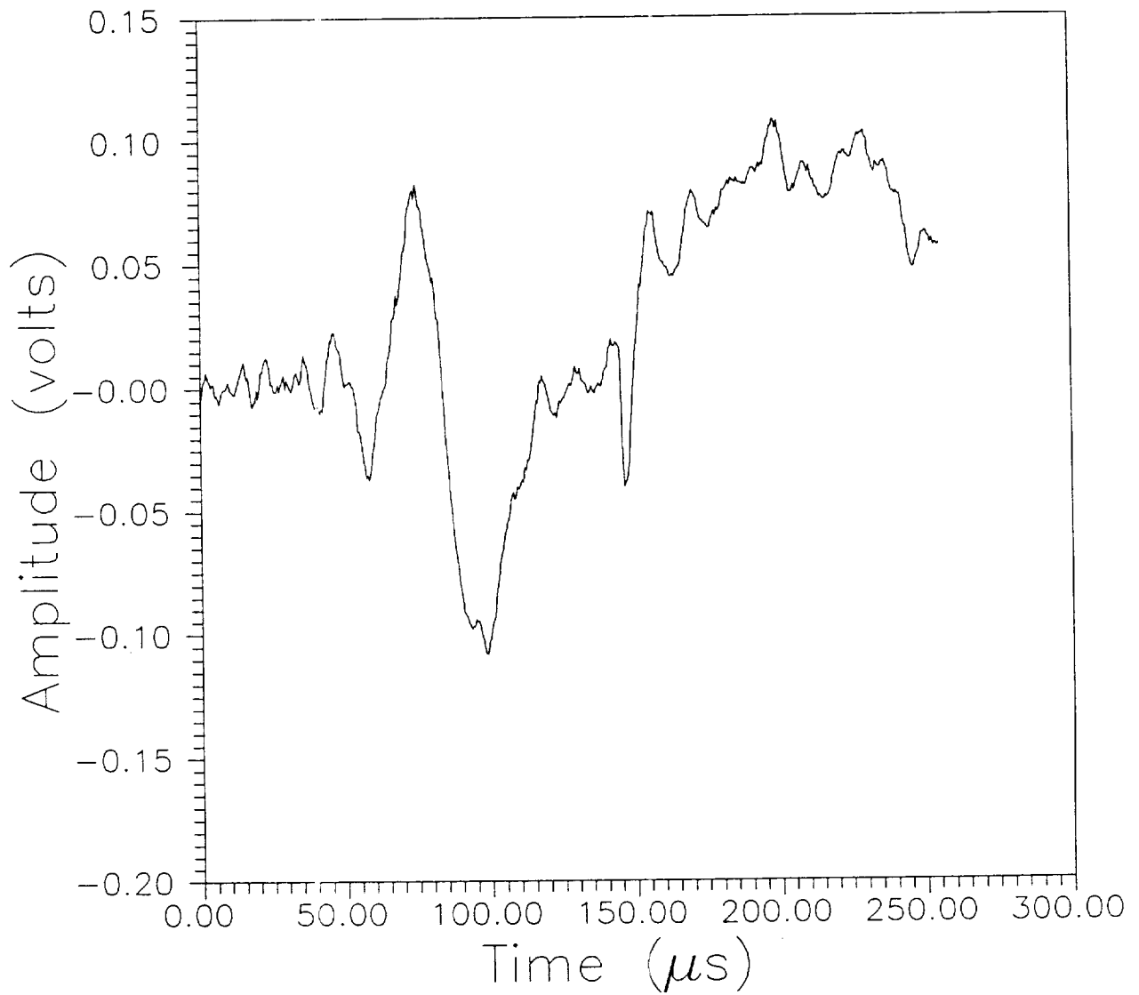
Figure 27. Pulsed laser generated fiber-optic heterodyne laser interferometer detected waveform for the graphite/epoxy 90 degree laminate specimen.
