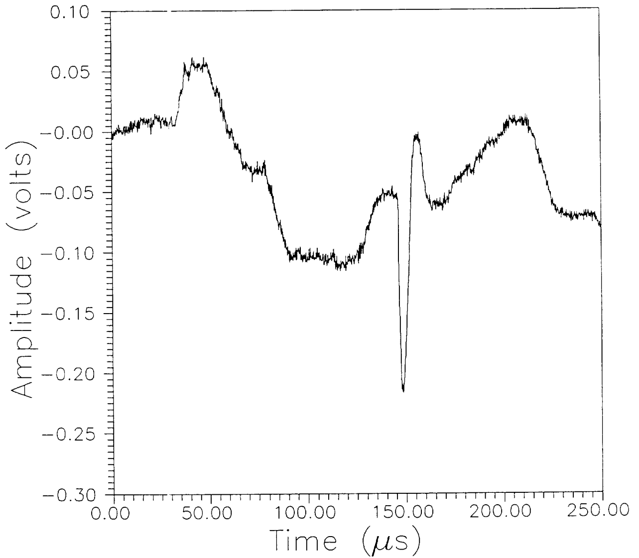
Figure 31. Pulsed laser generated fiber-optic heterodyne laser interferometer detected waveform for the filament wound composite specimen.
