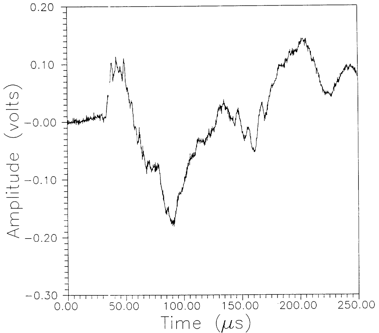
Figure 32. Pulsed laser generated conical point piezoelectric transducer detected waveform for the filament wound composite specimen.
