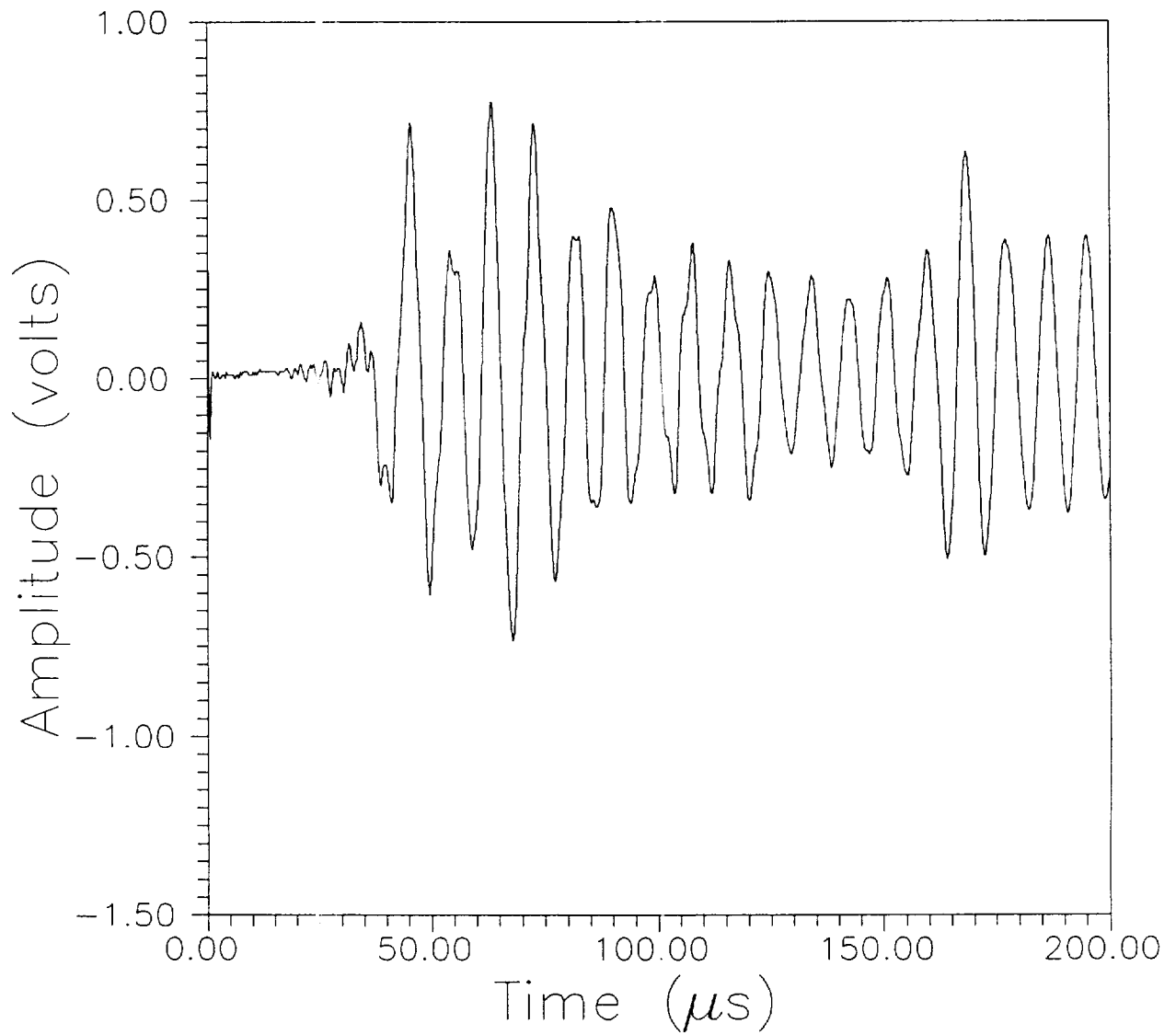
Figure 34. AET 206 AU unit detected waveform for the graphite/epoxy cross-ply laminate specimen.
