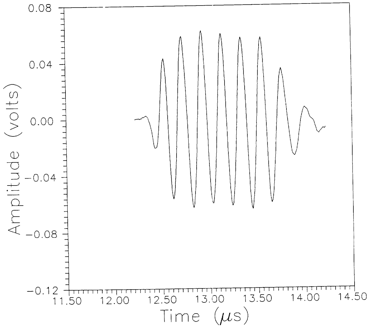
Figure 12. Ultrasonic waveform detected using experimental arrangement shown in Figure 11.
