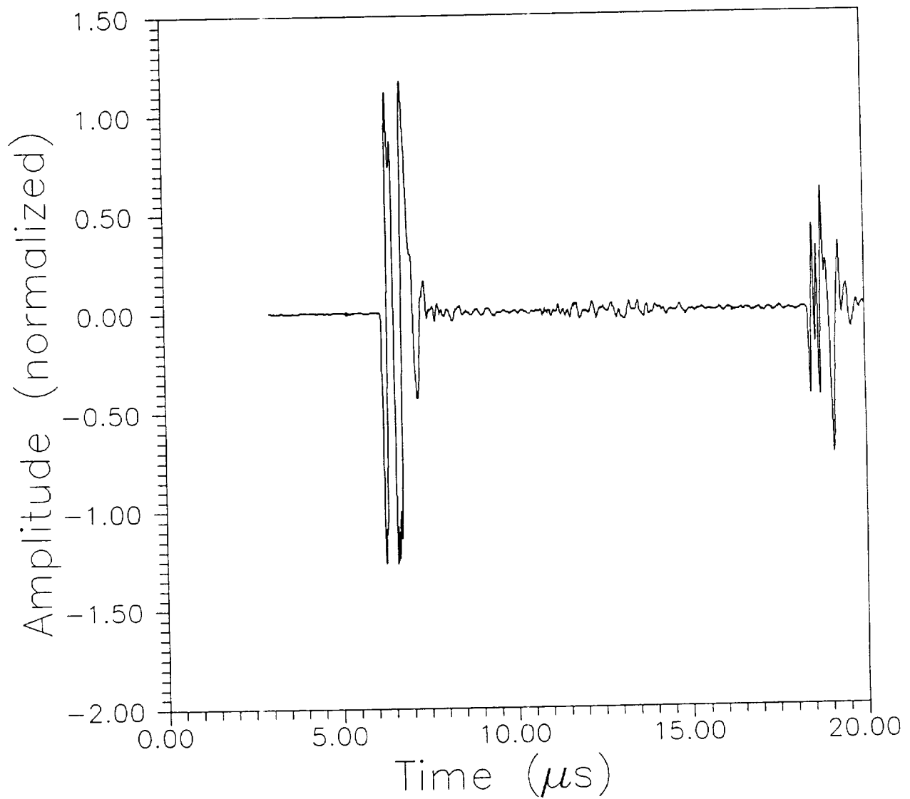
Figure 21. Waveform obtained for pulsed laser generated ultrasound in aluminum block detected by 2.25 MHz piezoelectric transducer on epicenter.
