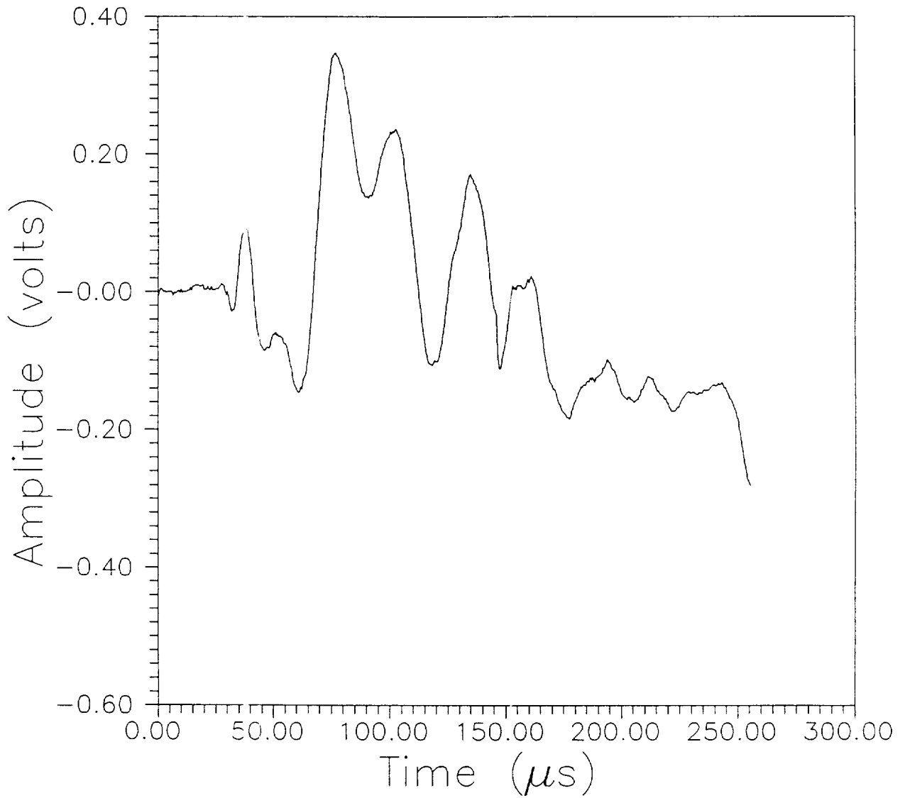
Figure 29. Pulsed laser generated fiber-optic heterodyne laser interferometer detected waveform for the graphite/epoxy cross-ply laminate specimen.
