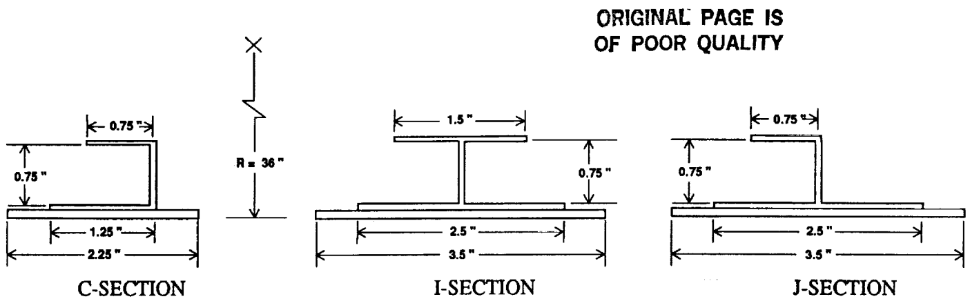
(a) Cross-sectional dimensions.
