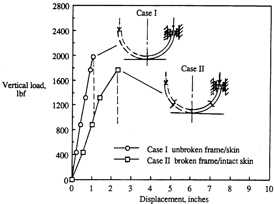
(a) Load-displacement.
