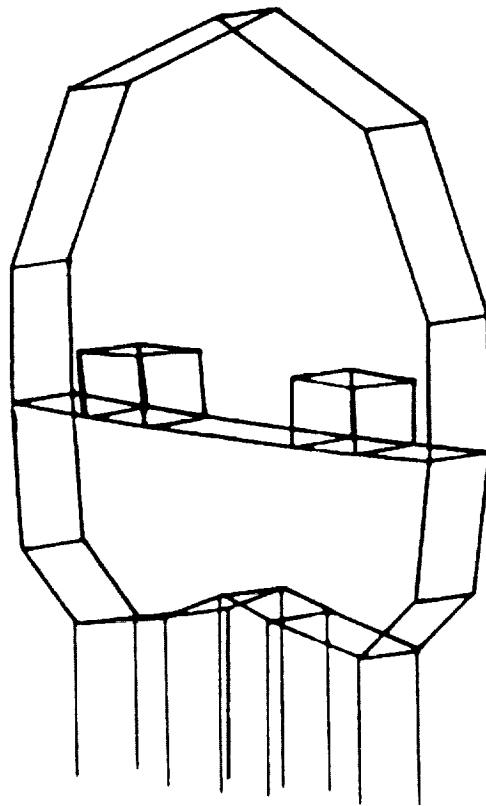
Figure 10.-Computer graphics showing analytical failure of metal transport section.
