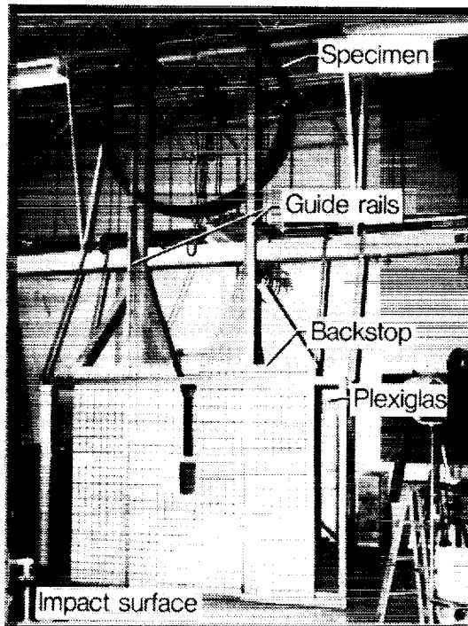
Figure 6. - Composite Z-frame in drop apparatus.
