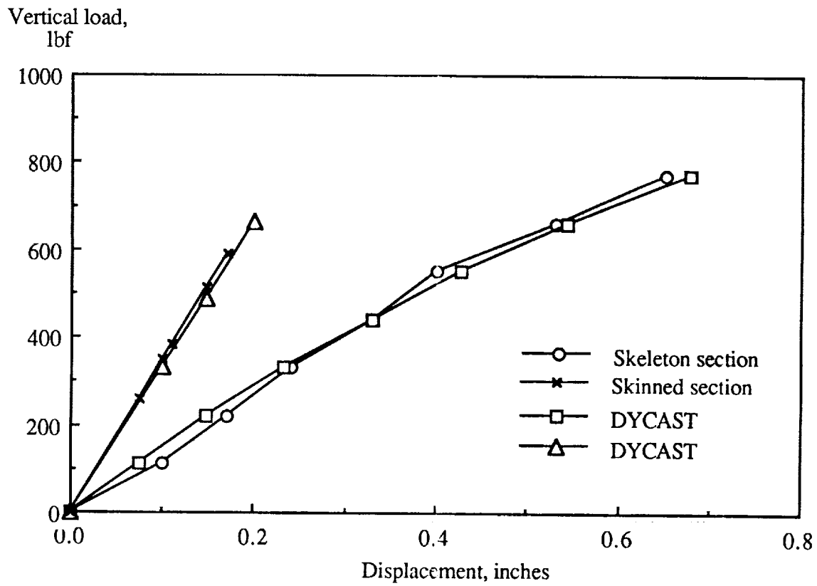
Figure 17. - Comparison of experimental and analytical stiffness of skeleton and skinned composite subfloors.
