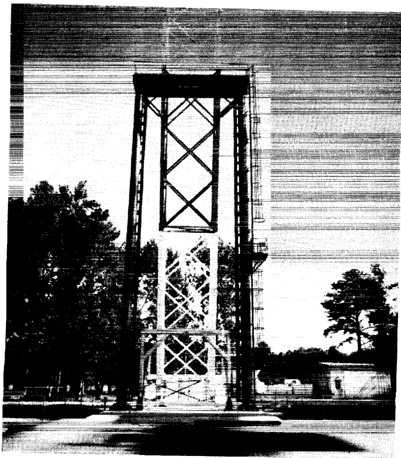
Figure 3. - 70 Foot Vertical Drop Test Apparatus.
