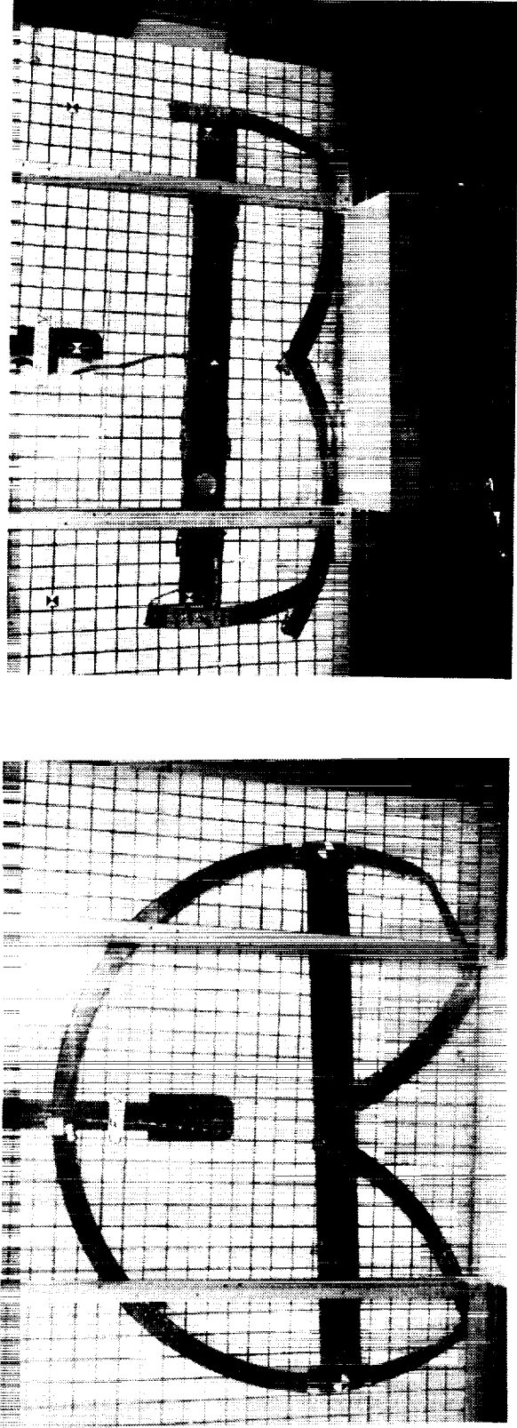
(a) Photographs of failed frames.
