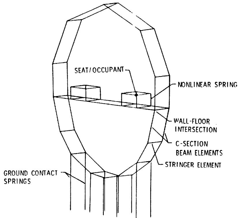
Figure 9. - Finite element two-frame model of metal transport section.
