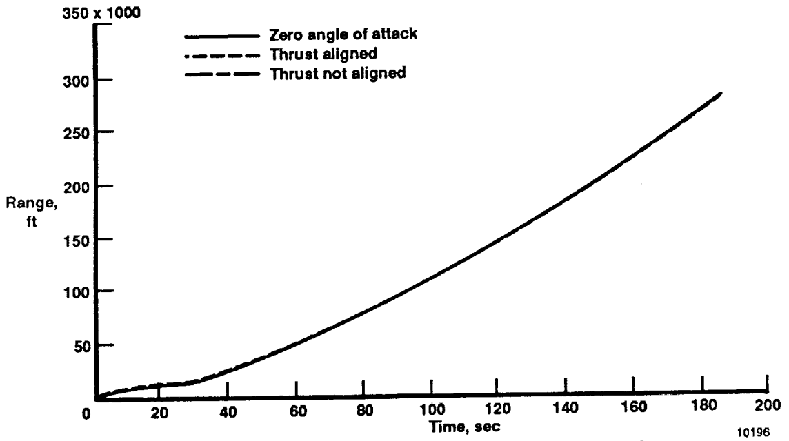
(a) Range as a function of time. Figure 7. Effects of equations of motion.
