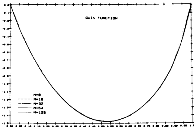
Figure 6 Gain Function k_{2,\alpha}^2(\cdot) ( \alpha = 0.3, C = I )
