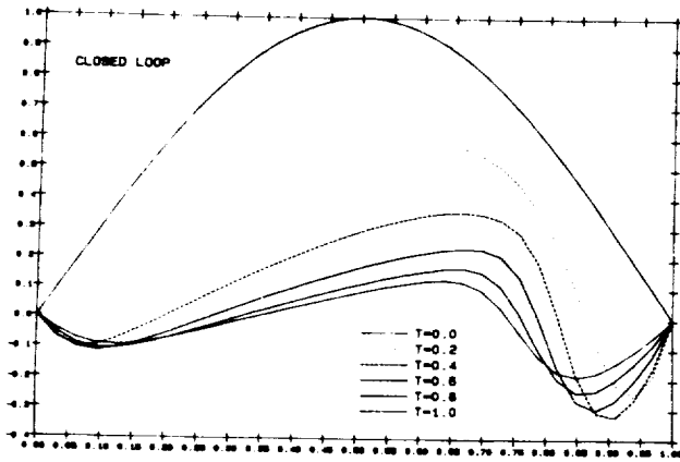
Figure 13 Closed Loop (Re=100, feedback by k_{a,n}^1(\cdot) )
