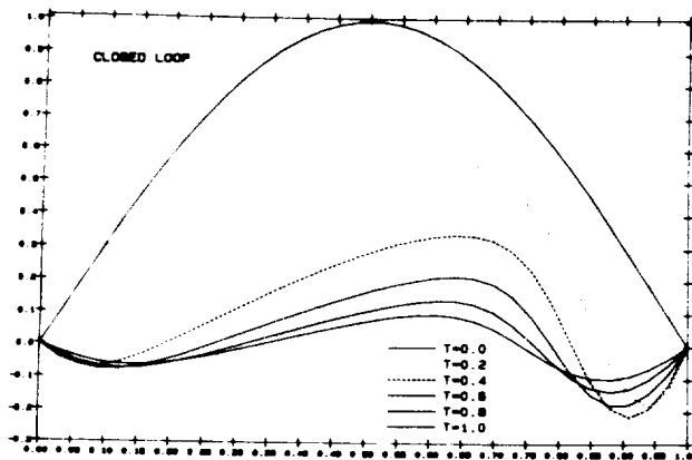
Figure 3 Closed Loop (feedback by k_{2,\alpha}^1(\cdot) )
