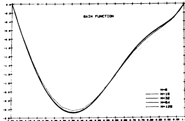
Figure 8 Gain Function k_{0,x}^1(.) ( \alpha = 0.6, C = 1 )
