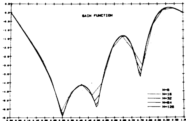
Figure 4 Gain Function k_{2,\alpha}^2(\cdot) ( \alpha = 0.6, C(z) = (z(0.3), z(0.5), z(0.75)) )
