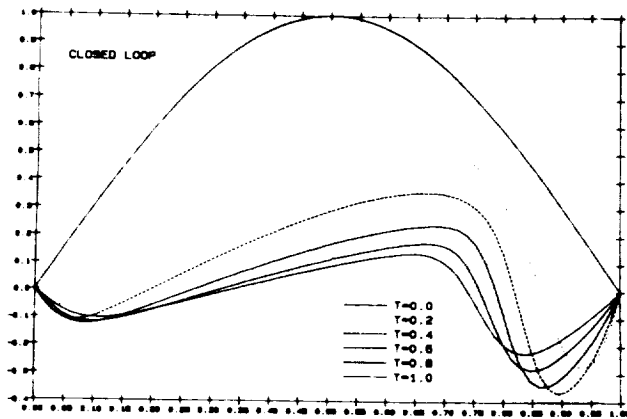
Figure 15 Closed Loop (N=64, Re=120, feedback by k_{a,n}^1(\cdot) )
