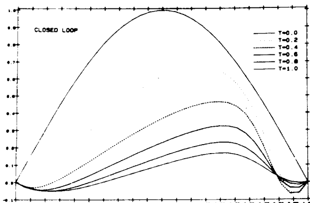
Figure 9 Closed Loop (feedback by k_{0,x}^1(.) )
