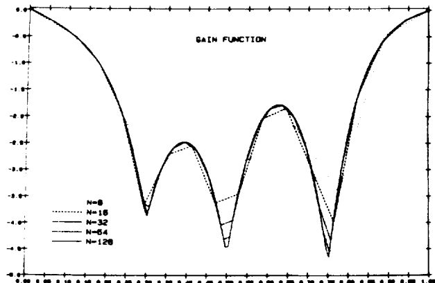
Figure 2 Gain Function k_{2,\alpha}^1(\cdot) ( \alpha = 0.3, C(z) = (z(0.3), z(0.5), z(0.75)) )
