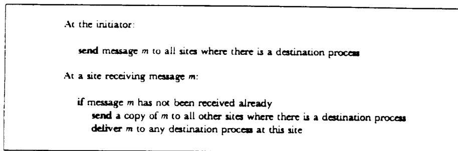
Figure 14.3 A simple atomic broadcast protocol
