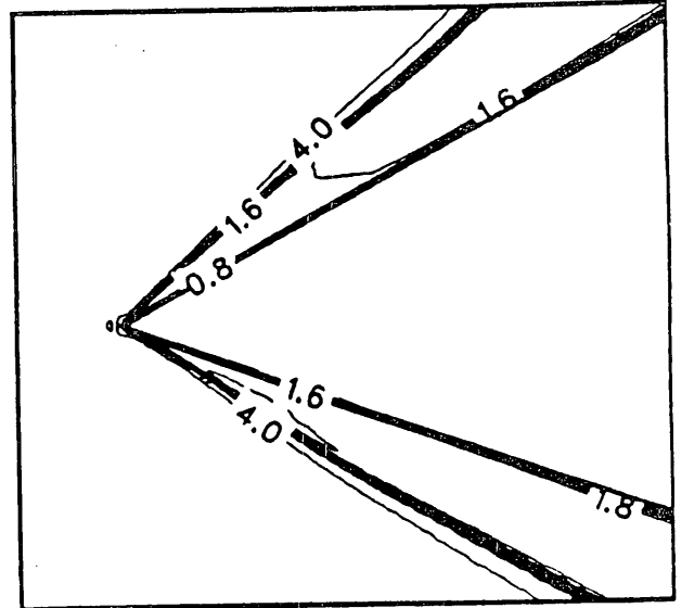
Fig. 8. Mach number contours for reacting stoichiometric air-fuel mixture flowing over wedge at Mach 4.2. The rotation of the wave with combustion indicates a detonation.
