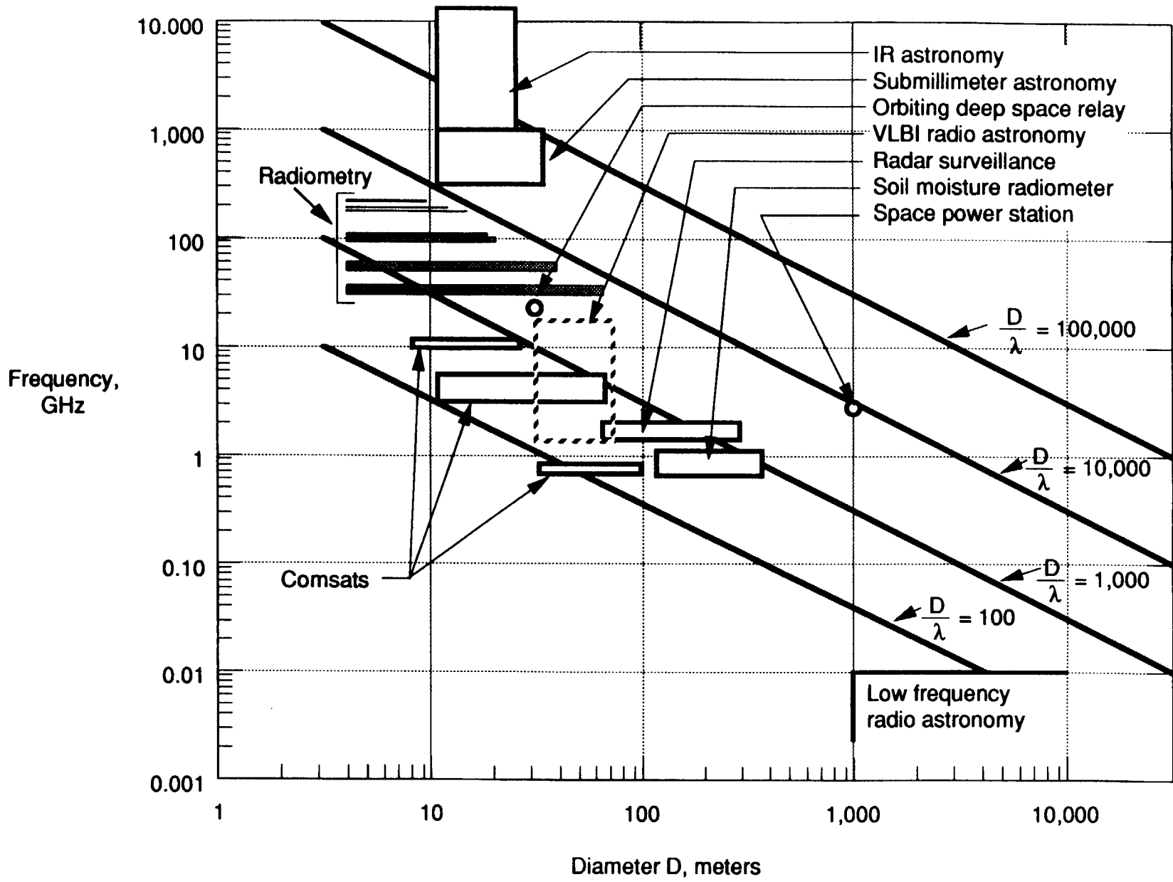
Figure 1. Large space antenna requirements.
