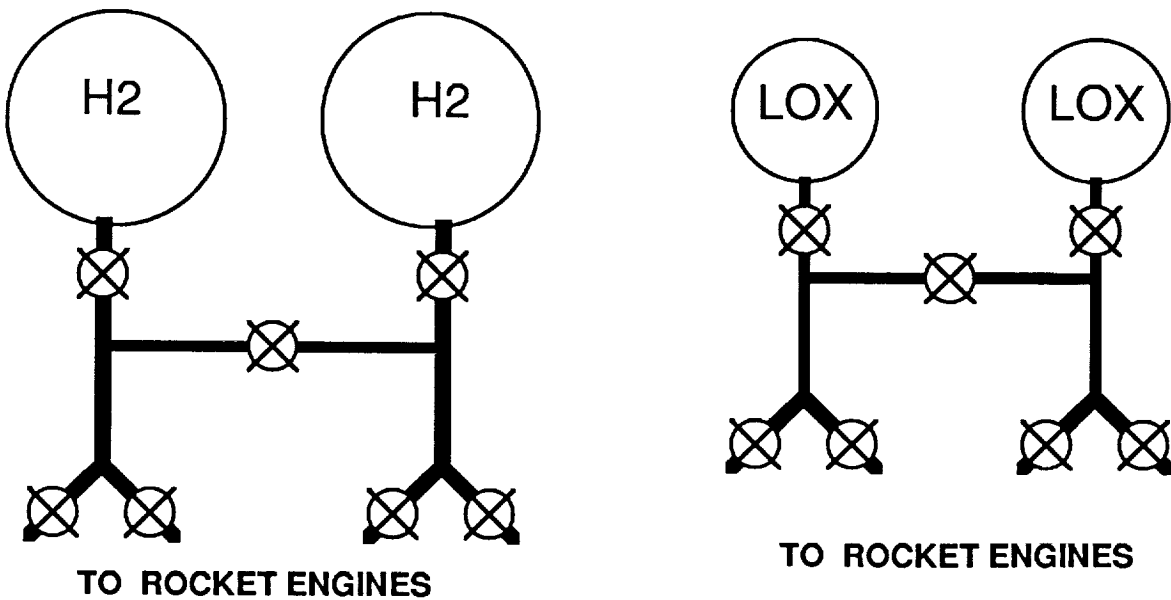
SCHEMATIC (DOUBLE REDUNDANCY)
