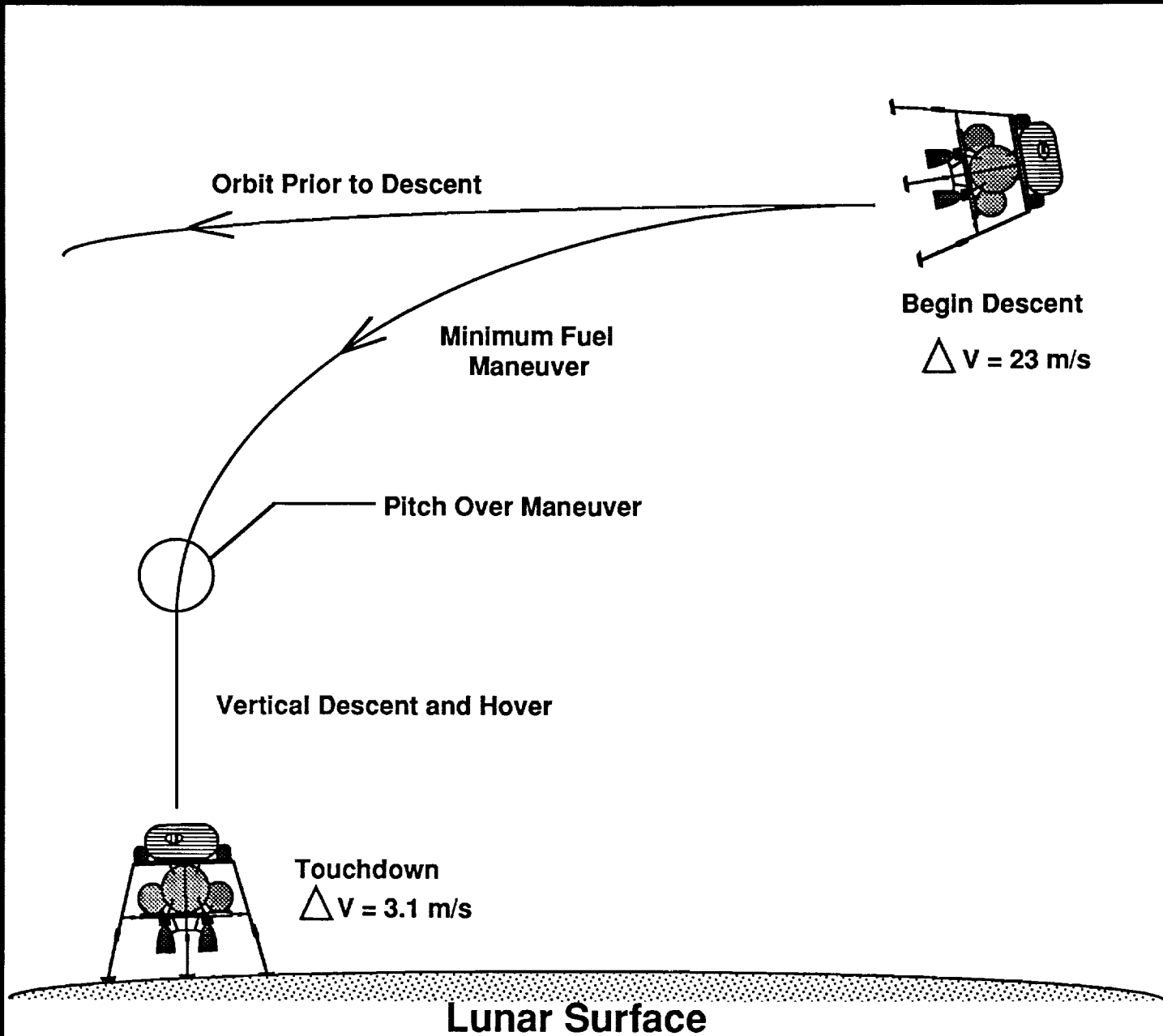
Fig. 3.3: Touchdown Sequence
