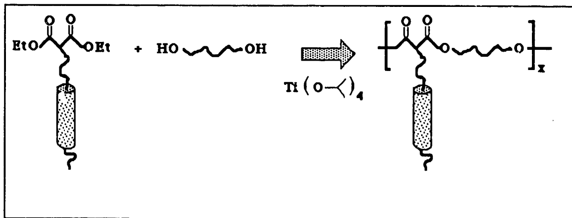
FIGURE 2.11 Preparation of sidechain LCPs by polyesterification.
