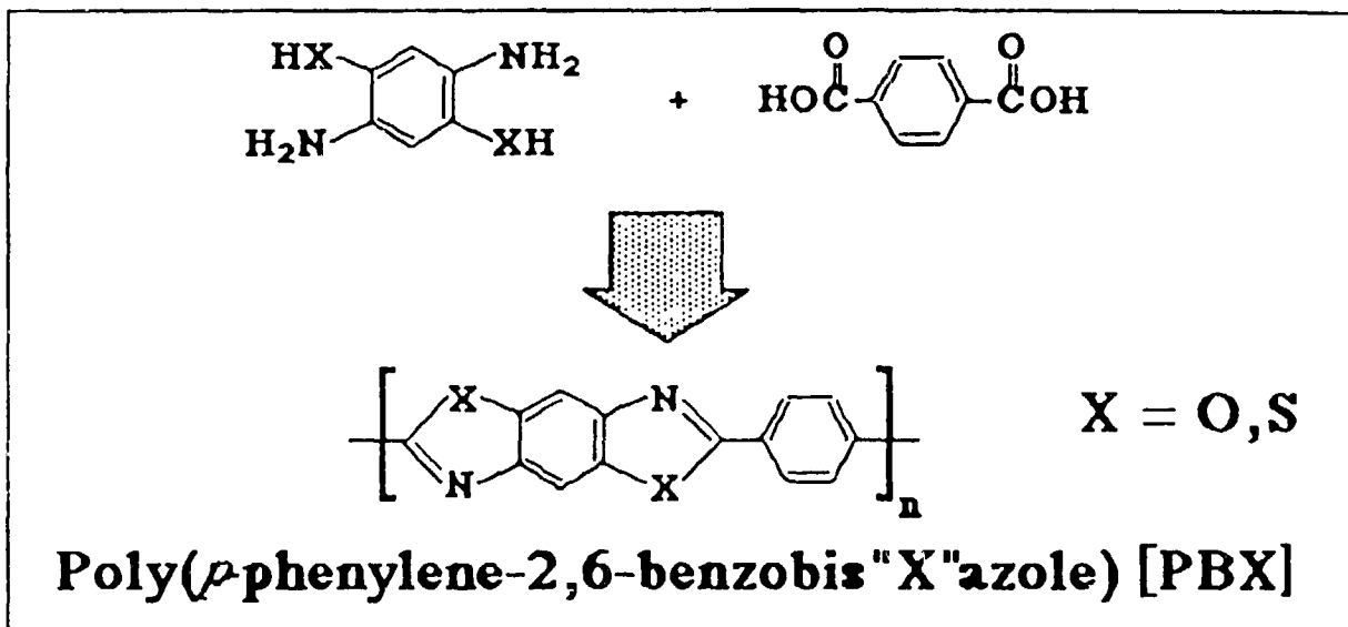
FIGURE 2.9 Synthesis of PBX polymers.
