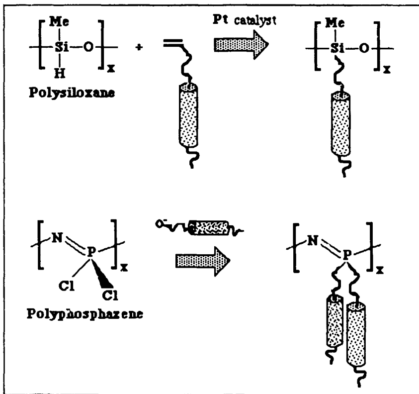
FIGURE 2.12 Examples of preparation of sidechain LCPs by derivatization of preformed polymers.
