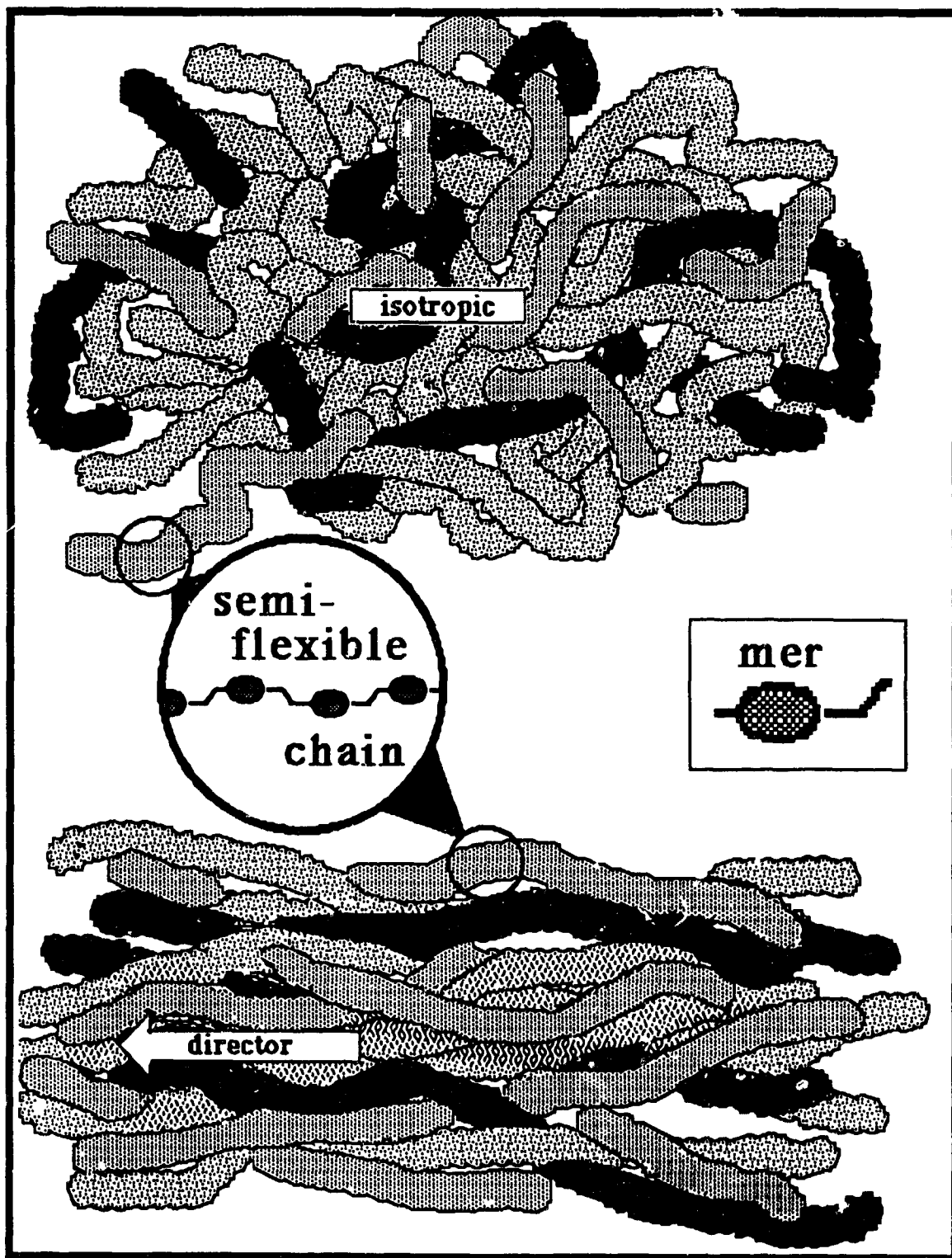
FIGURE 2.1 Schematic indication of the differences between an isotropic (top) and a liquid crystalline (bottom) polymer fluid.
