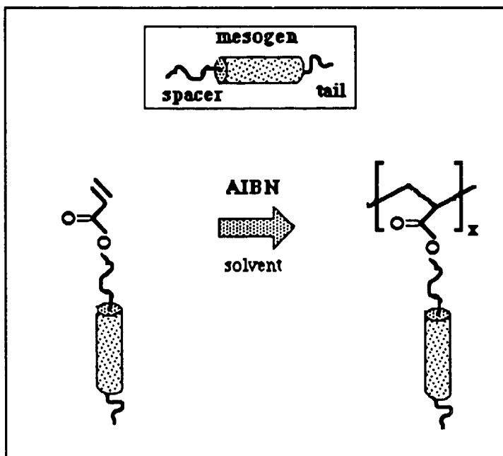
FIGURE 2.10 Preparation of sidechain LCPs by free radical polymerization.
