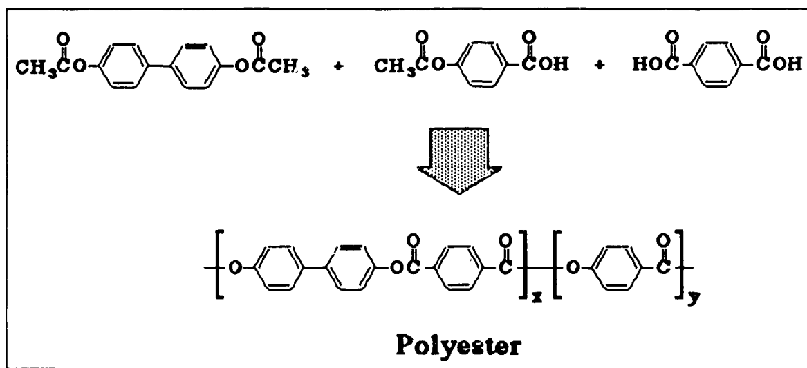
FIGURE 2.5 Condensation polymerization involving acidolysis.
