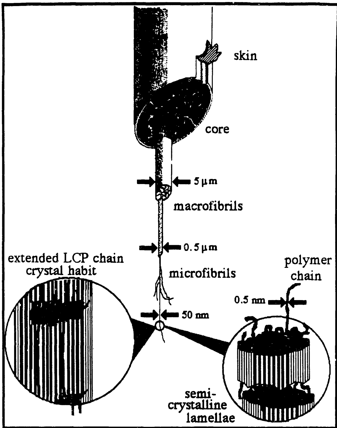
FIGURE 2.13 Hierarchical morphology in fibers.
