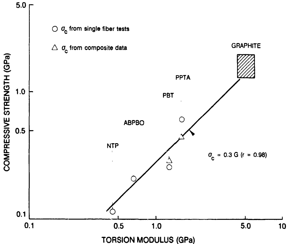
FIGURE 4.1 Compressive strength versus torsion modulus for some rigid rod polymers.
