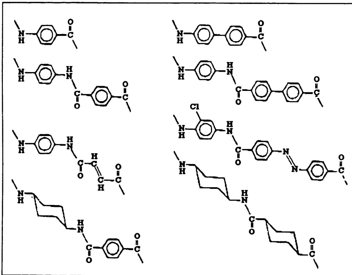
FIGURE 2.8 Lyotropic polyamide unit structures.
