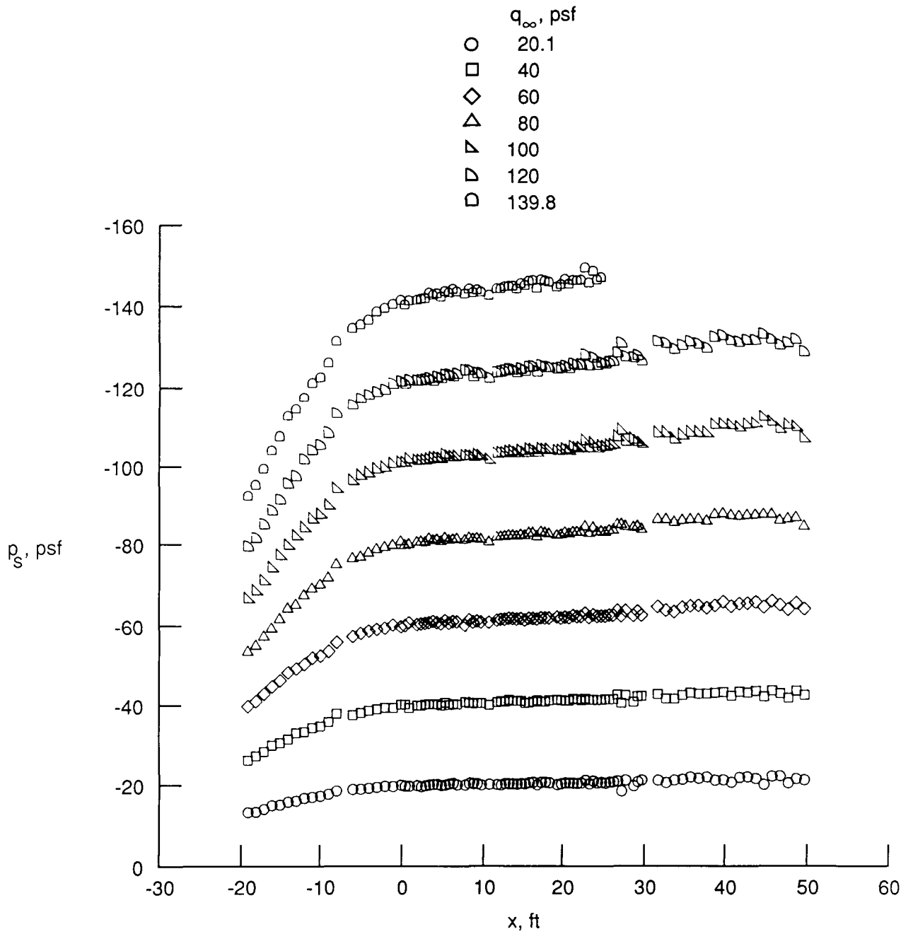
Figure 16. Longitudinal dynamic pressure distribution along centerline of closed test-section configuration with no floor boundary-layer control.
