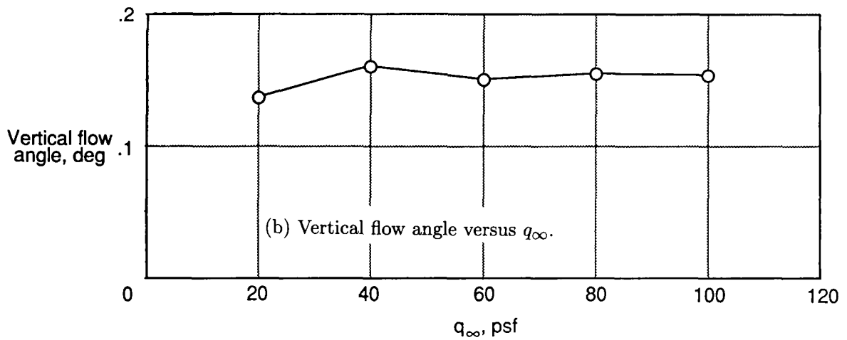
Figure 30. Measurements of vertical flow angle using lift data of an elliptical wing at q_\infty = 60 psf.
