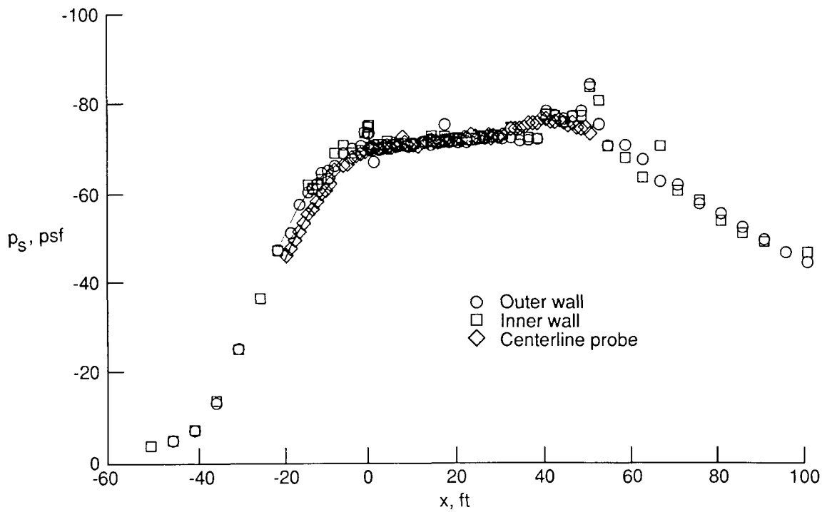
Figure 23. Static pressure data from tunnel stations -50 to 100 for closed test-section configuration with q_\infty = 70 psf.
