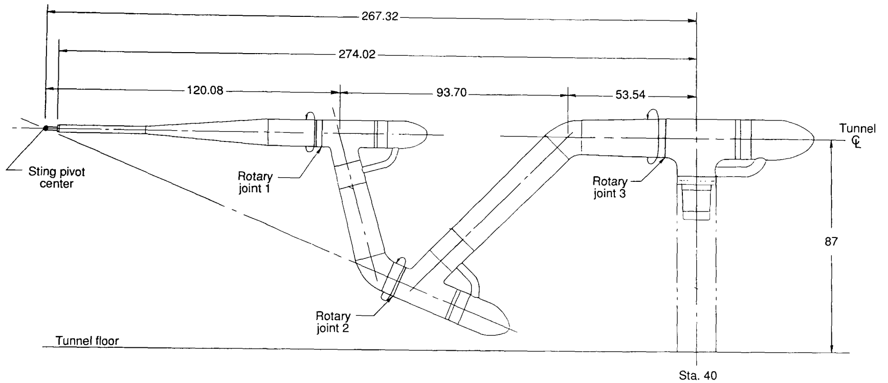
(c) \alpha - \beta sting used on cart 4.
