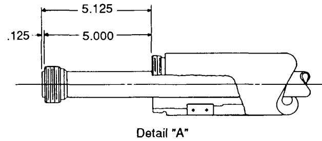
(b) Bent air sting using 729-type balances.
