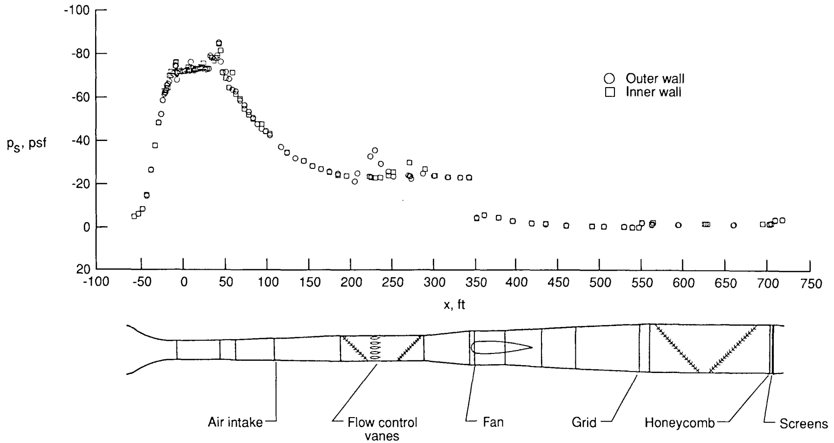
Figure 26. Static pressure distribution around entire tunnel circuit for closed test-section configuration with q_\infty = 70 psf.
