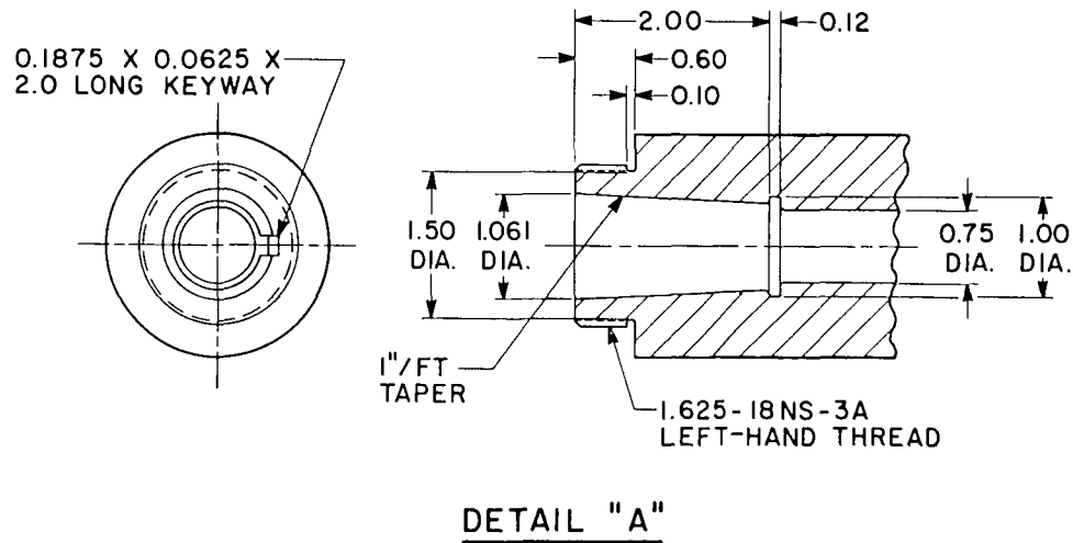
(a) Used with 708-type balances.
