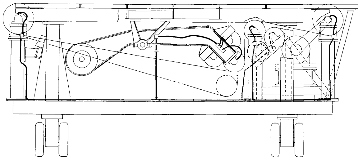
(a) Schematic of moving-belt cart.
