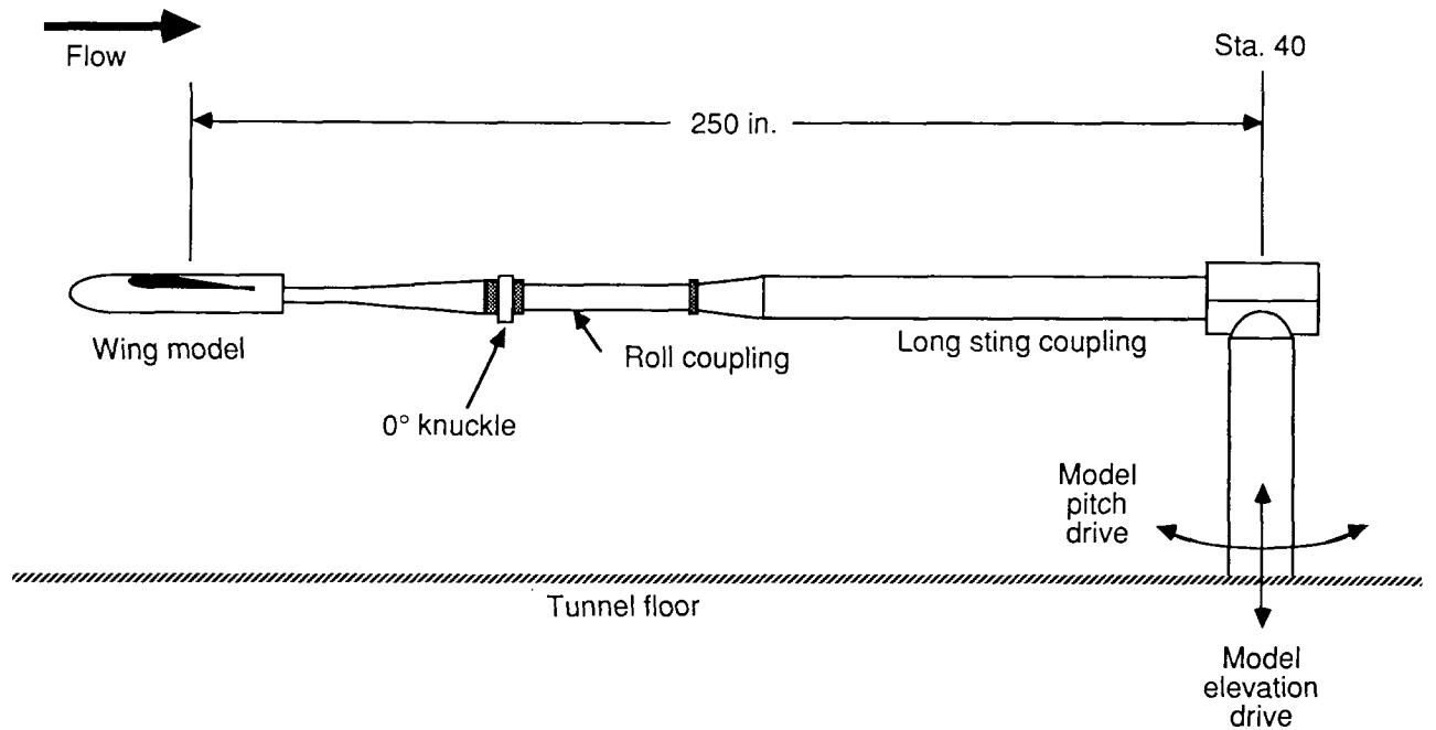
Figure 29. Sketch of elliptical wing model mounted in the 14- by 22-Foot Tunnel.
