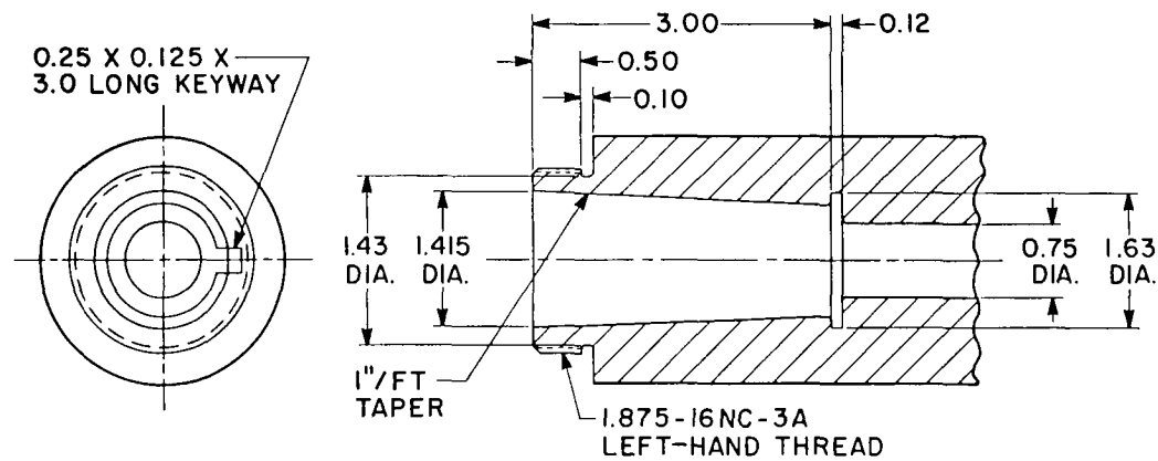
DETAIL "A"
