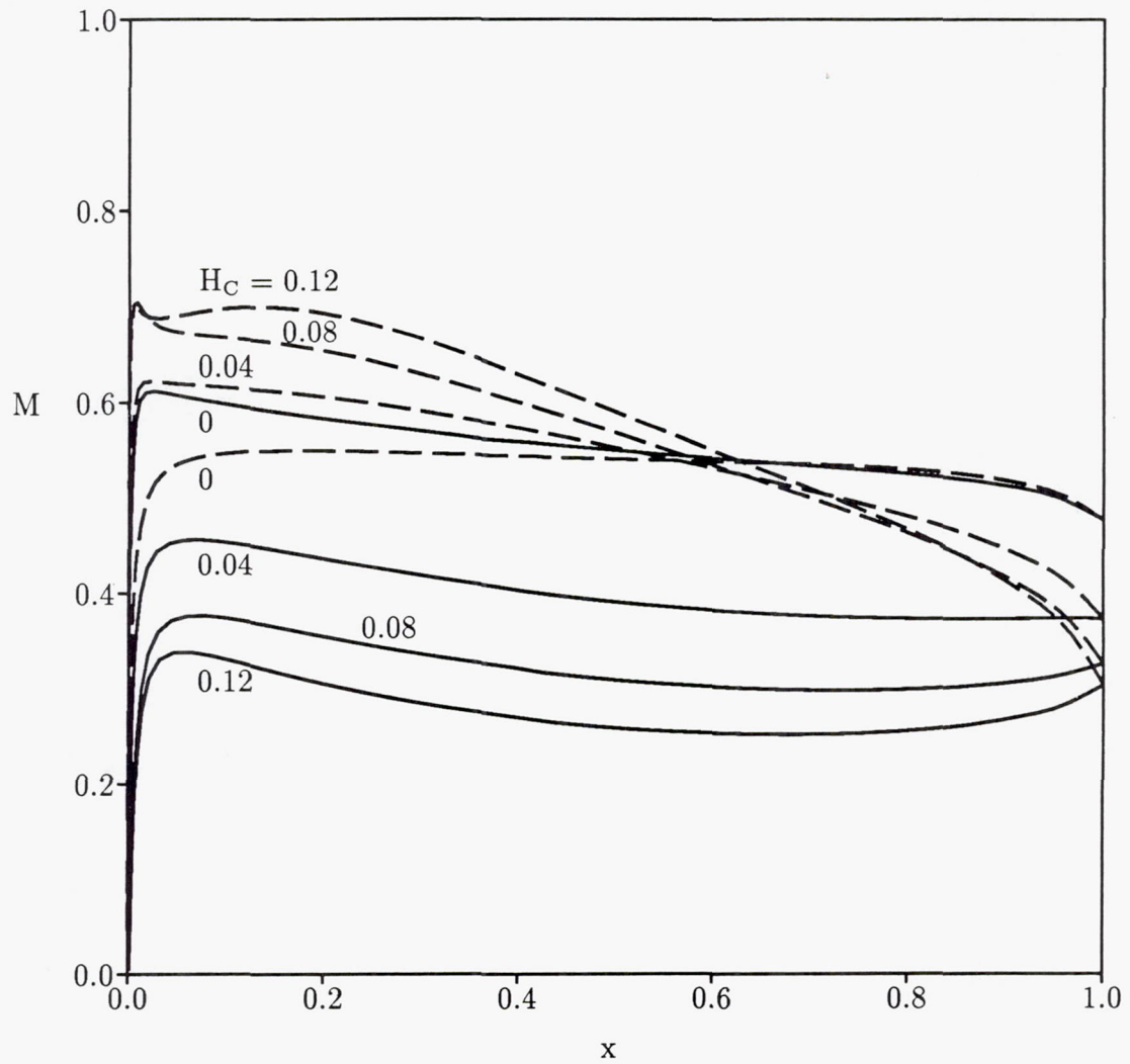
Figure 9 Effect of mean blade loading on the steady Mach number distribution along a blade surface for cascades of cambered NACA 0006 airfoils; - - - upper surface of blade, — lower surface.
