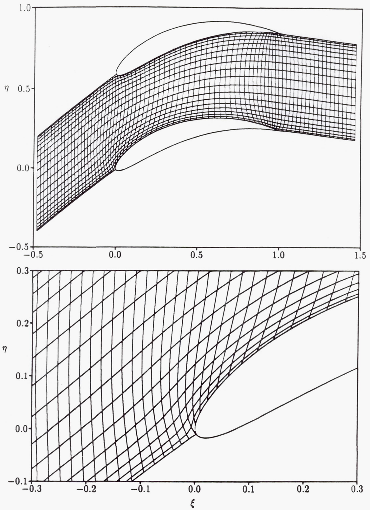
Figure 3. Extended blade-passage solution domain and computational grid.
