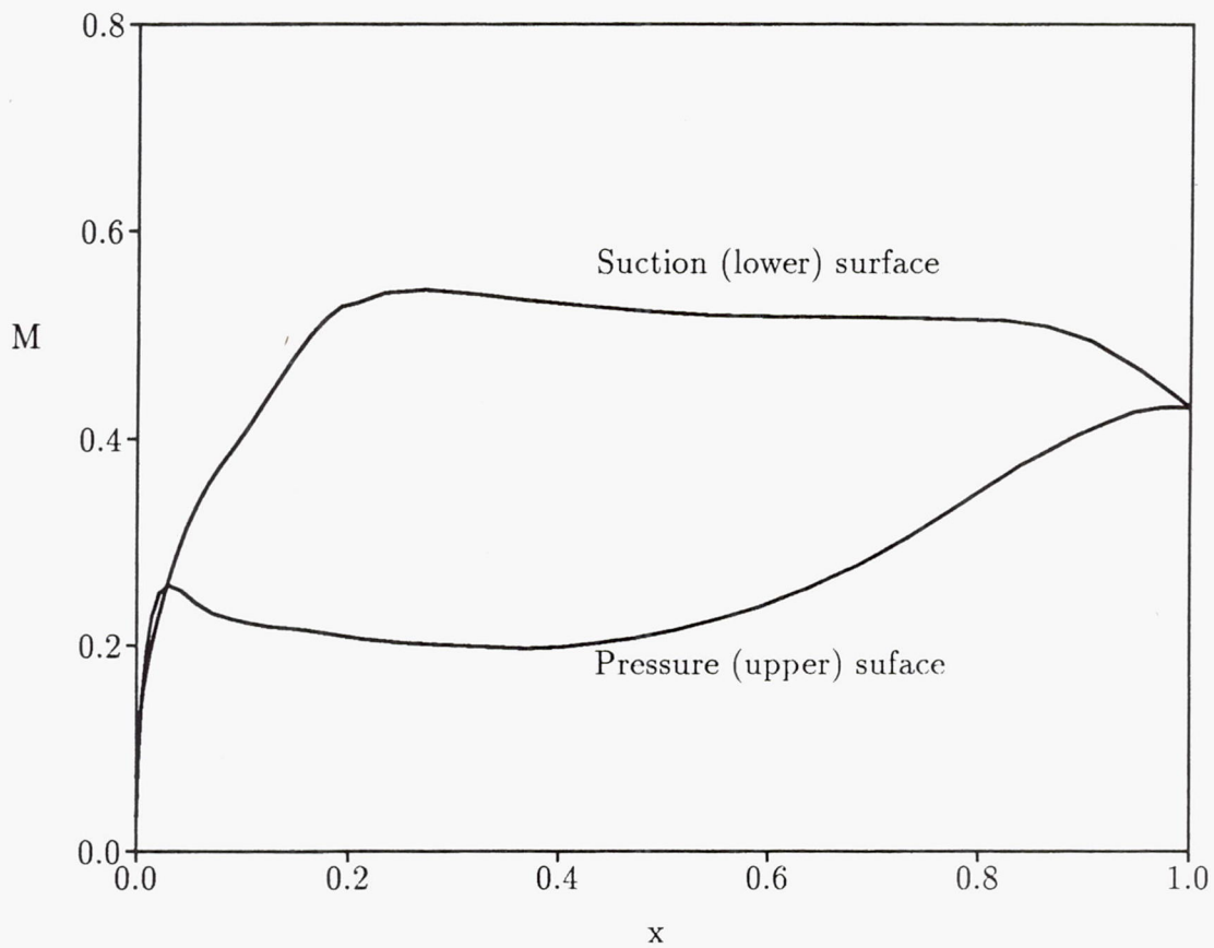
Figure 23. Mach number contours and surface Mach number distributions for steady flow with M_{\infty} = 0.19 and \Omega_{\infty} = 45 deg through the turbine cascade ( \Theta = 56.6 deg and G = 0.76 ).
