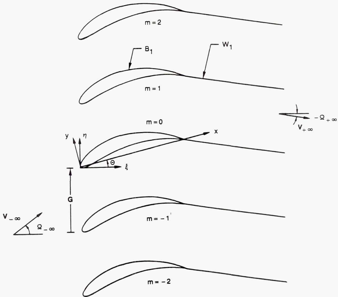
Figure 1. Two-dimensional compressor cascade.
