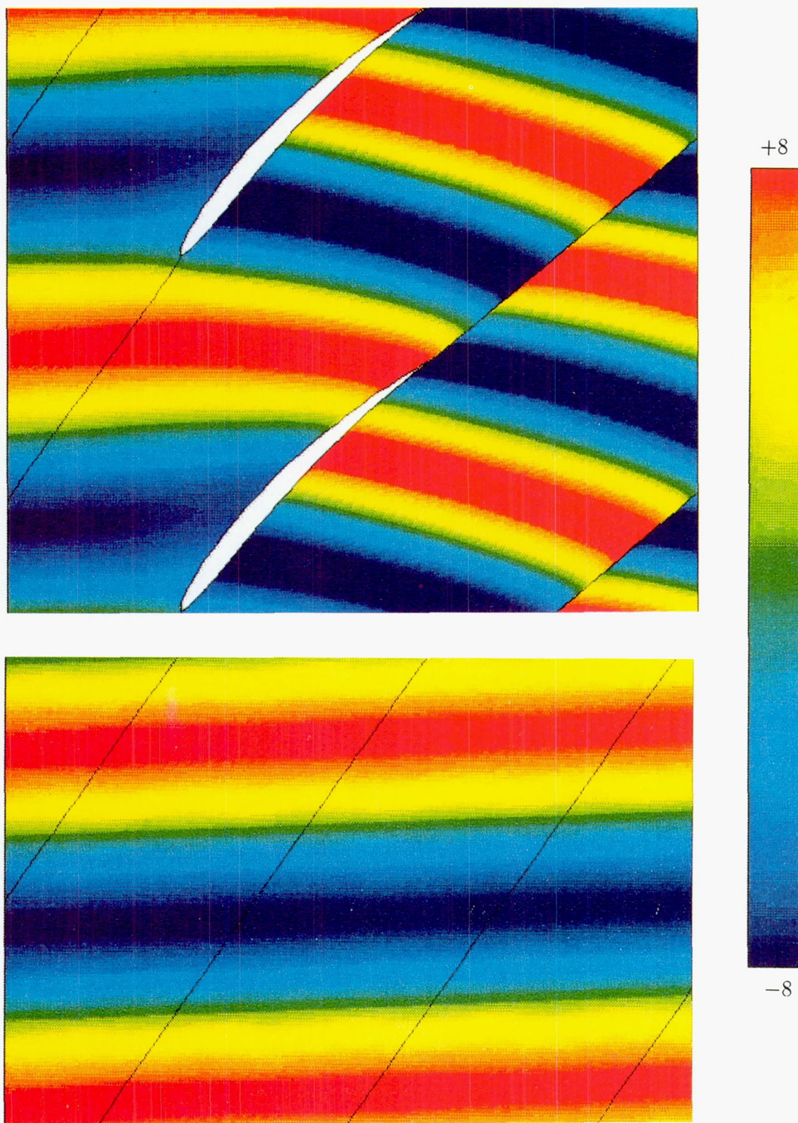
Figure 18. Contours of the real part of the unsteady vorticity for the cambered NACA 0006 and the corresponding flat-plate ( M = 0.7 , \Omega = \Theta = 55 deg, G = 1.0 ) cascades subjected to an incident vortical gust with v_g = (1, 0) , \omega = 5 and \sigma = -2\pi .
