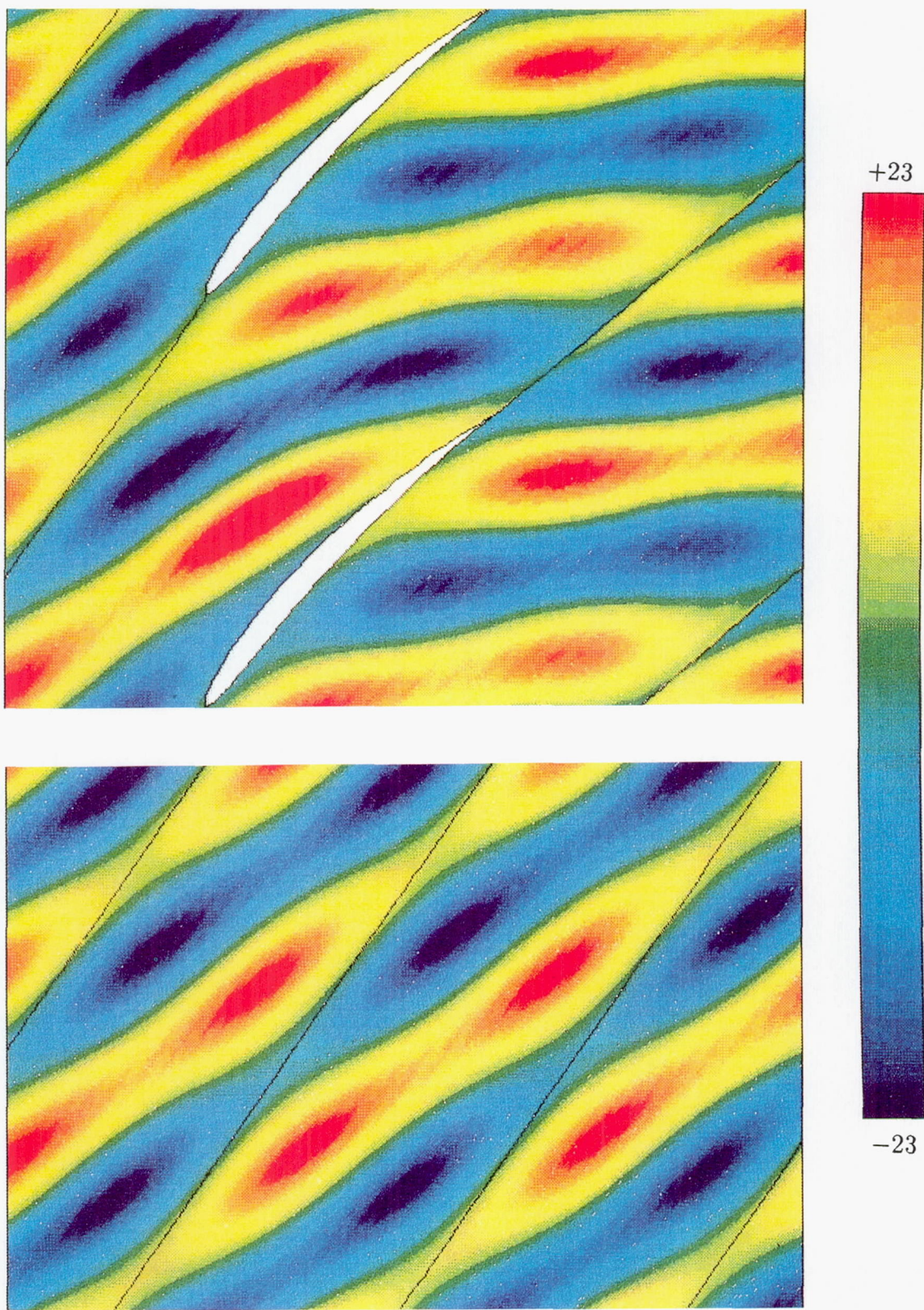
Figure 19. Contours of the real part of the source term for the cambered NACA 0006 and the corresponding flat-plate cascades subjected to an incident vortical gust with v_g = (1, 0) , \omega = 5 and \sigma = -2\pi .
