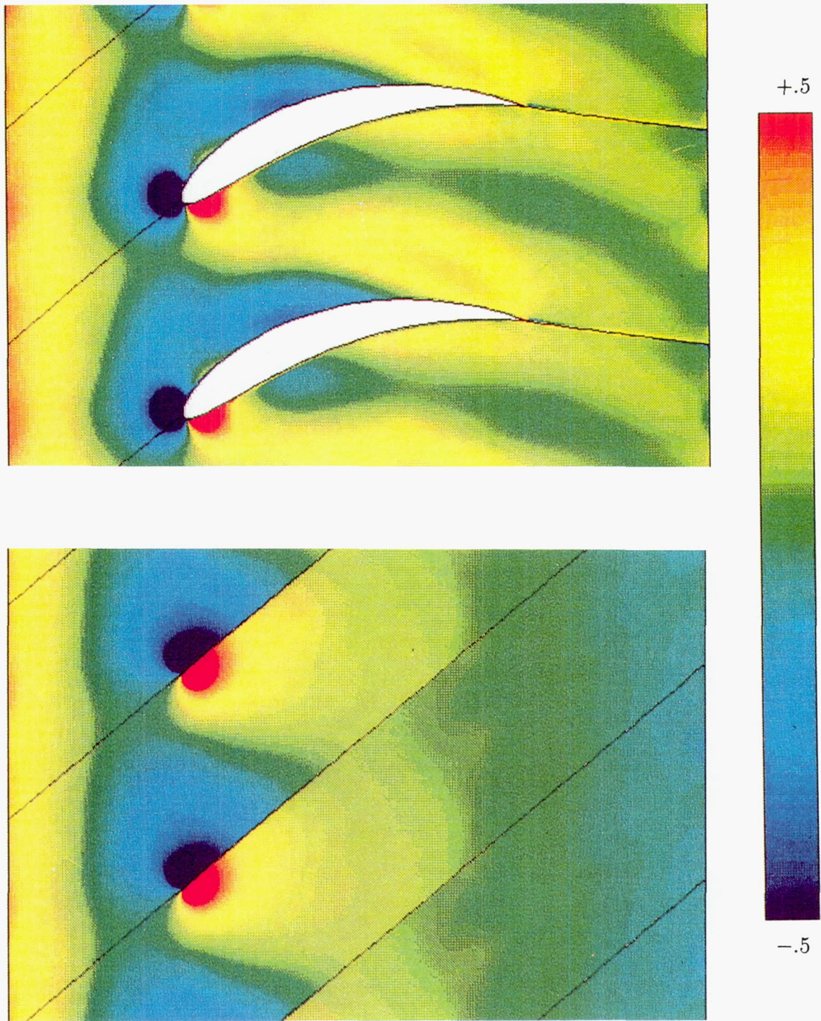
Figure 14. Contours of the in-phase component (real part) of the unsteady pressure for the EGV and the corresponding flat-plate cascades subjected to an incident vortical gust with \mathbf{v}_g = (1, 0) , \omega = 5 and \sigma = -2\pi .
