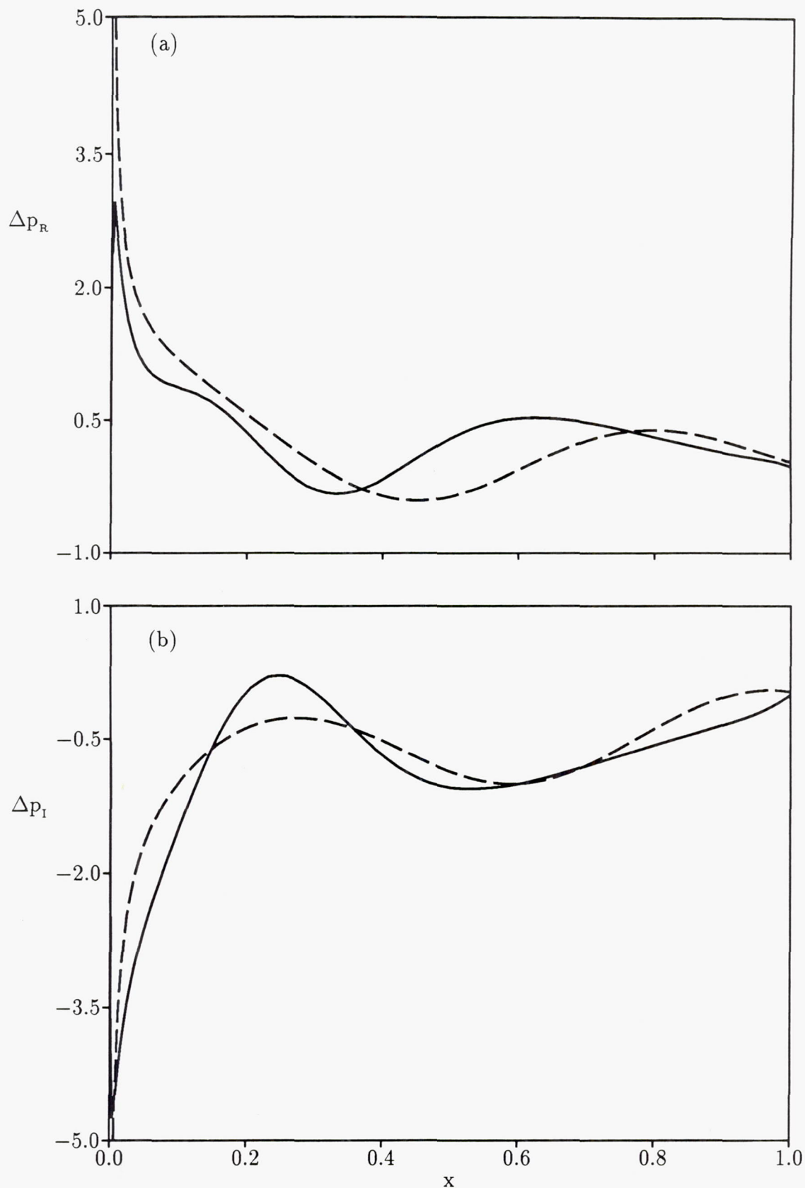
Figure 21. Unsteady pressure-difference response for the cambered NACA 0006 and corresponding flat-plate cascades subjected to an incident vortical gust with v_g = (1, 0) , \omega = 5 and \sigma = -2\pi : (a) in-phase component (real part); (b) out-of-phase component (imaginary part); - - - flat-plate cascade, — NACA 0006 cascade.
