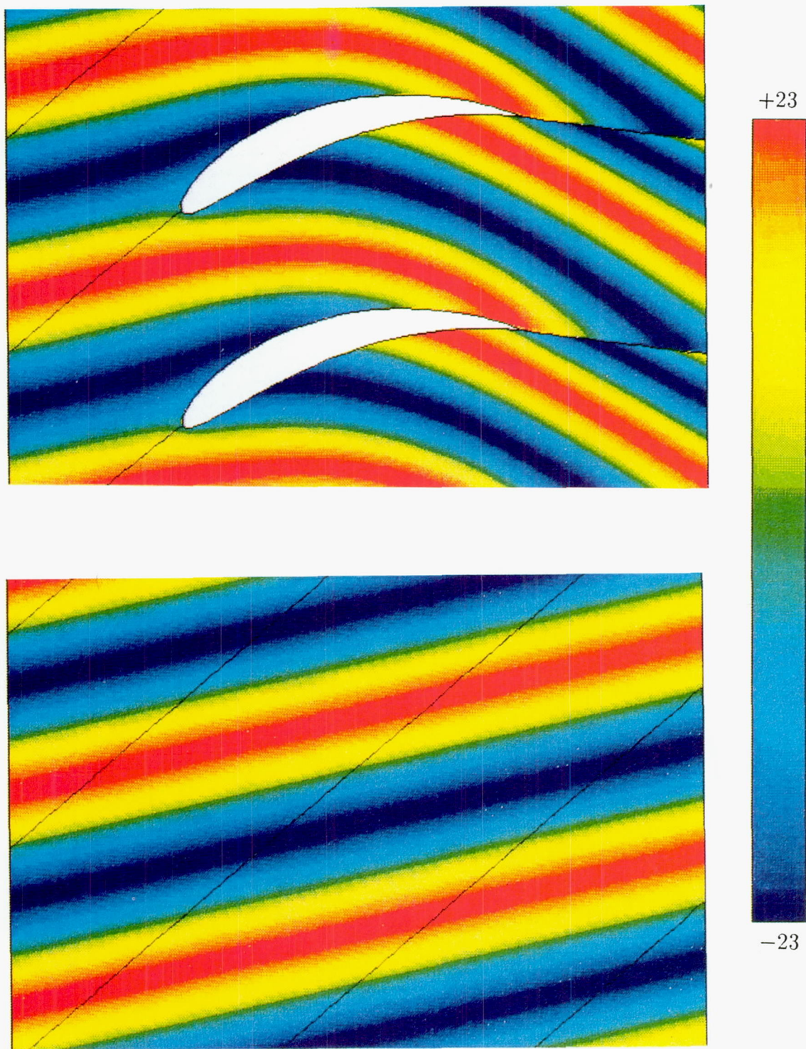
Figure 12. Contours of the real part of the unsteady vorticity for the EGV and the corresponding flat-plate ( M = 0.3 , \Omega = \Theta = 40 deg, G = 0.6 ) cascades subjected to an incident vortical gust with v_g = (1, 0) , \omega = 5 and \sigma = -2\pi .
