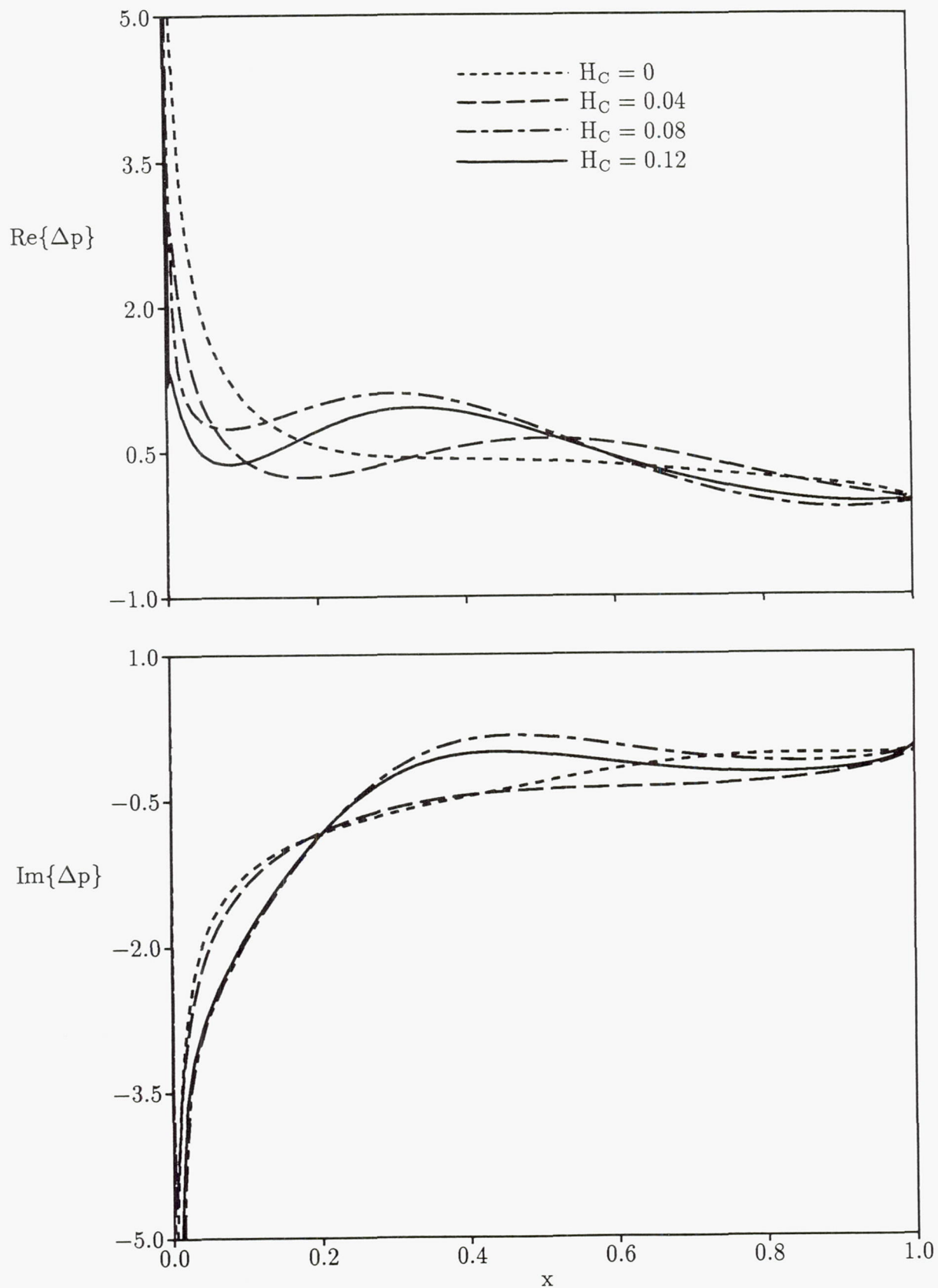
Figure 10. Effect of mean blade loading on the unsteady pressure-difference response for cascades of cambered NACA 0006 blades subjected to an incident vortical gust with v_g = (1, 0) , \omega = 5 and \sigma = -2\pi : (a) and (b) as in figure 5.
