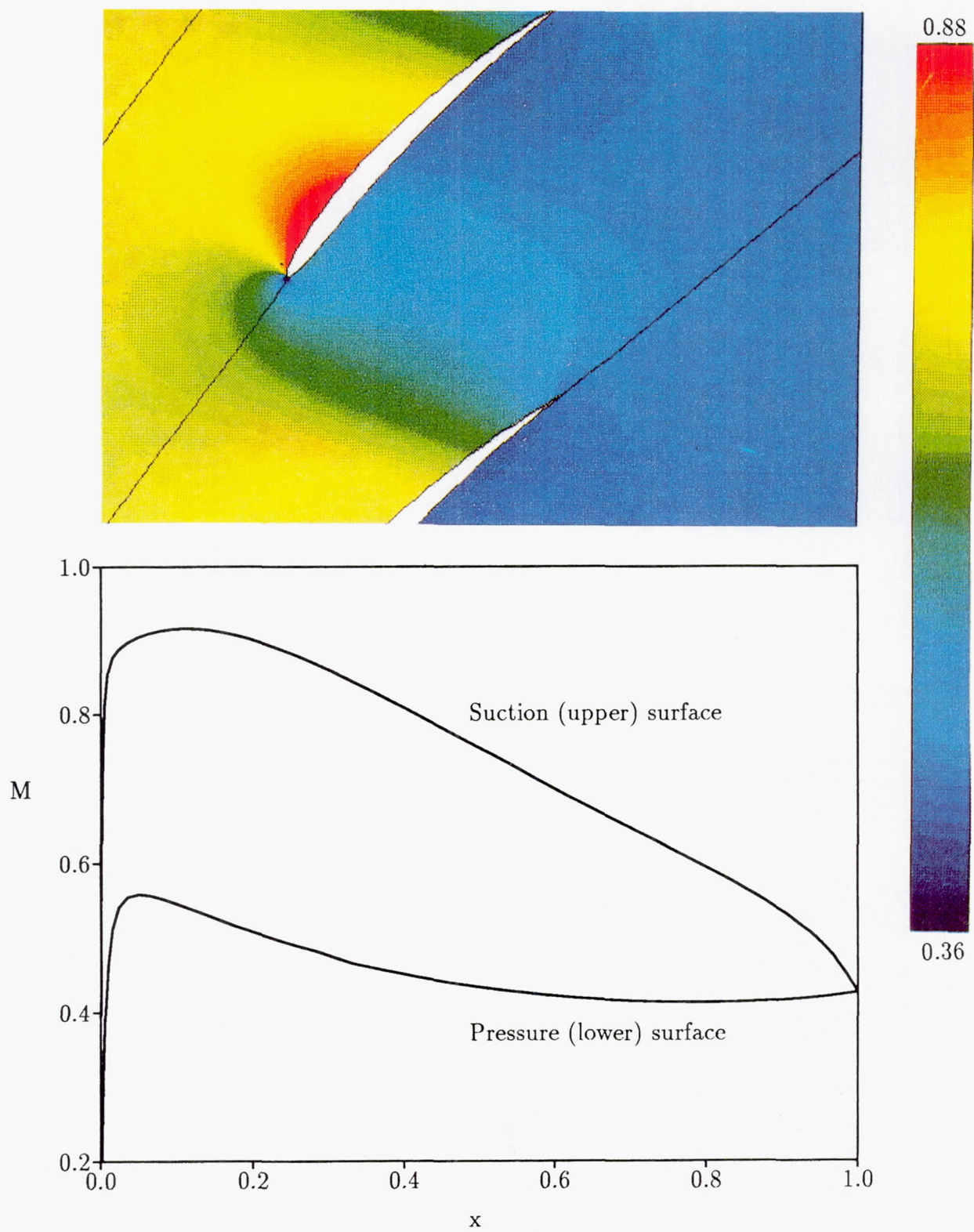
Figure 17. Mach number contours and surface Mach number distributions for steady flow with M_{-\infty} = 0.7 and \Omega_{-\infty} = 55 deg through the cambered NACA 0006 cascade ( \Theta = 45 deg, G = 1.0 , H_T = 0.06 and H_C = 0.05 ).
