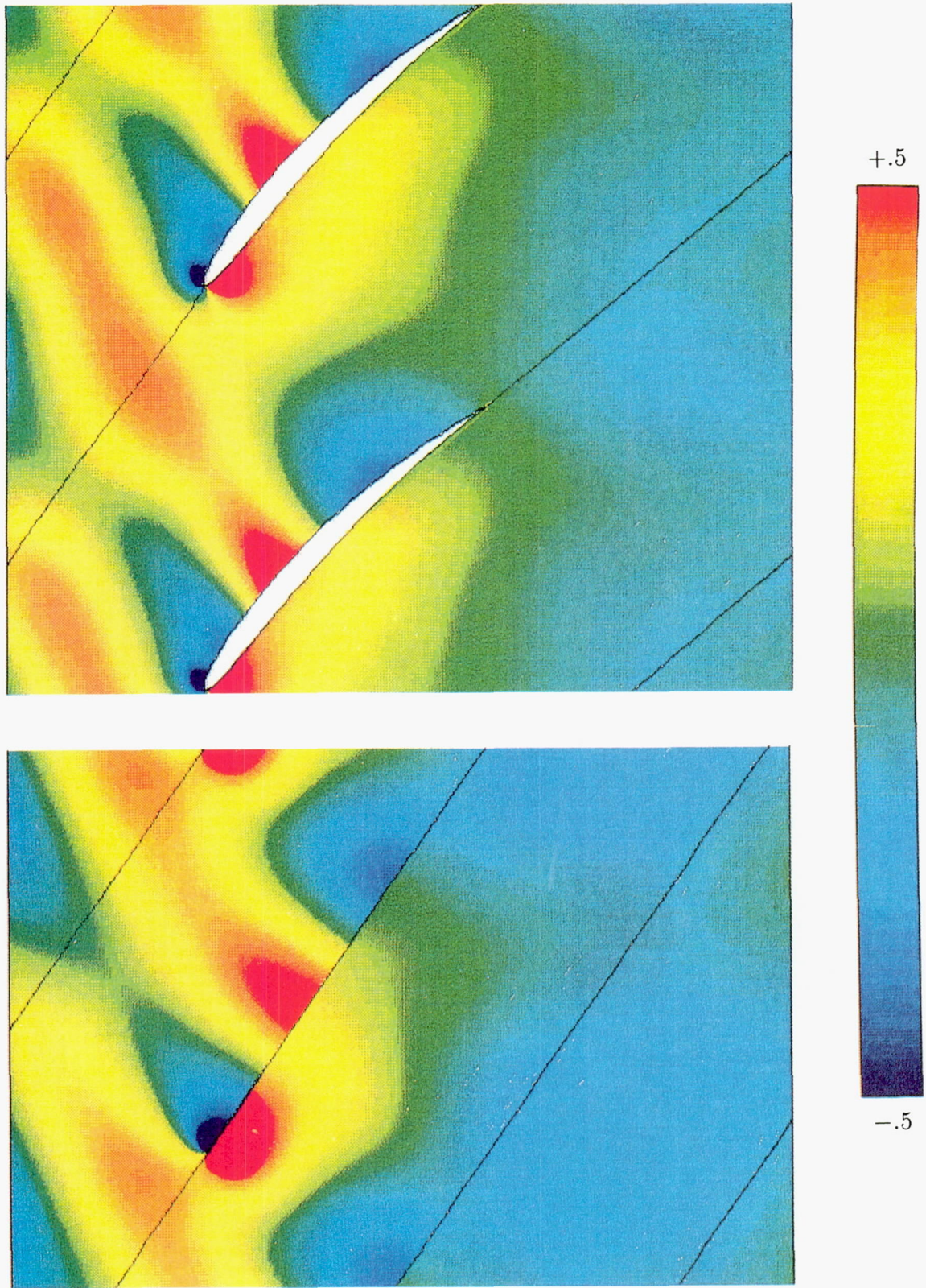
Figure 20. Contours of the in-phase component (real part) of the unsteady pressure for the cambered NACA 0006 and the corresponding flat-plate cascades subjected to an incident vortical gust with v_g = (1, 0) , \omega = 5 and \sigma = -2\pi .
