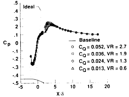
Figure 6. Pressure distributions for jet vortex generators with variable C_Q for D_o/\theta = 0.48 , \alpha = 45^\circ , and \beta = 90^\circ
