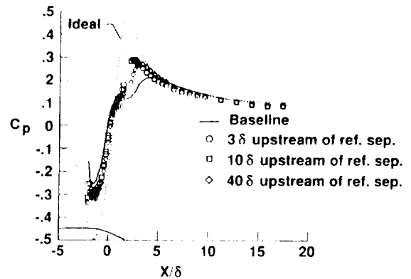
Figure 13. Pressure distributions for jet vortex generators at several streamwise locations with \alpha = 15^\circ , \beta = 90^\circ , D_o/\theta = 0.24 , VR = 6.8 , and C_Q = 0.034 .
