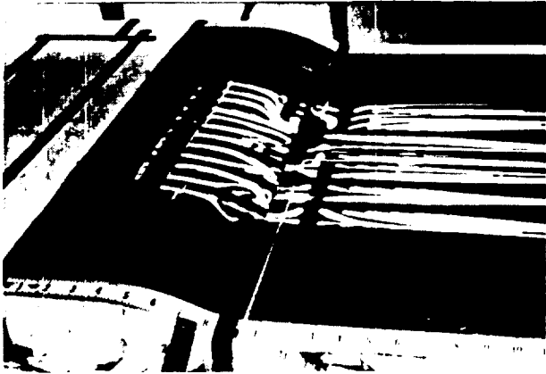
Figure 15. Oil flow visualization for counter-rotating jet vortex generators with \alpha = 45^\circ , \beta = \pm 90^\circ , D_o/\theta = 0.24 , VR = 6.8 , and C_Q = 0.034 .
