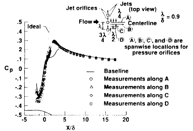
Figure 12. Pressure distributions for jet vortex generators at several spanwise locations with \alpha = 15^\circ , \beta = 90^\circ , D_o/\theta = 0.24 , VR = 6.8 , and C_Q = 0.034 .
