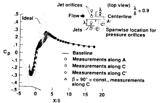
Figure 14. Pressure distributions at several spanwise locations for counter-rotating jet vortex generators with \alpha = 45^\circ , \beta = \pm 90^\circ , D_o/\theta = 0.24 , VR = 6.8 , and C_Q = 0.034 .
