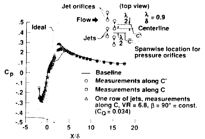
Figure 19. Pressure distributions at two spanwise locations for a double row of counter-rotating jet vortex generators with \alpha = 15^\circ , D_o/\theta = 0.24 , VR = 3.4 , and C_Q = 0.017 .
