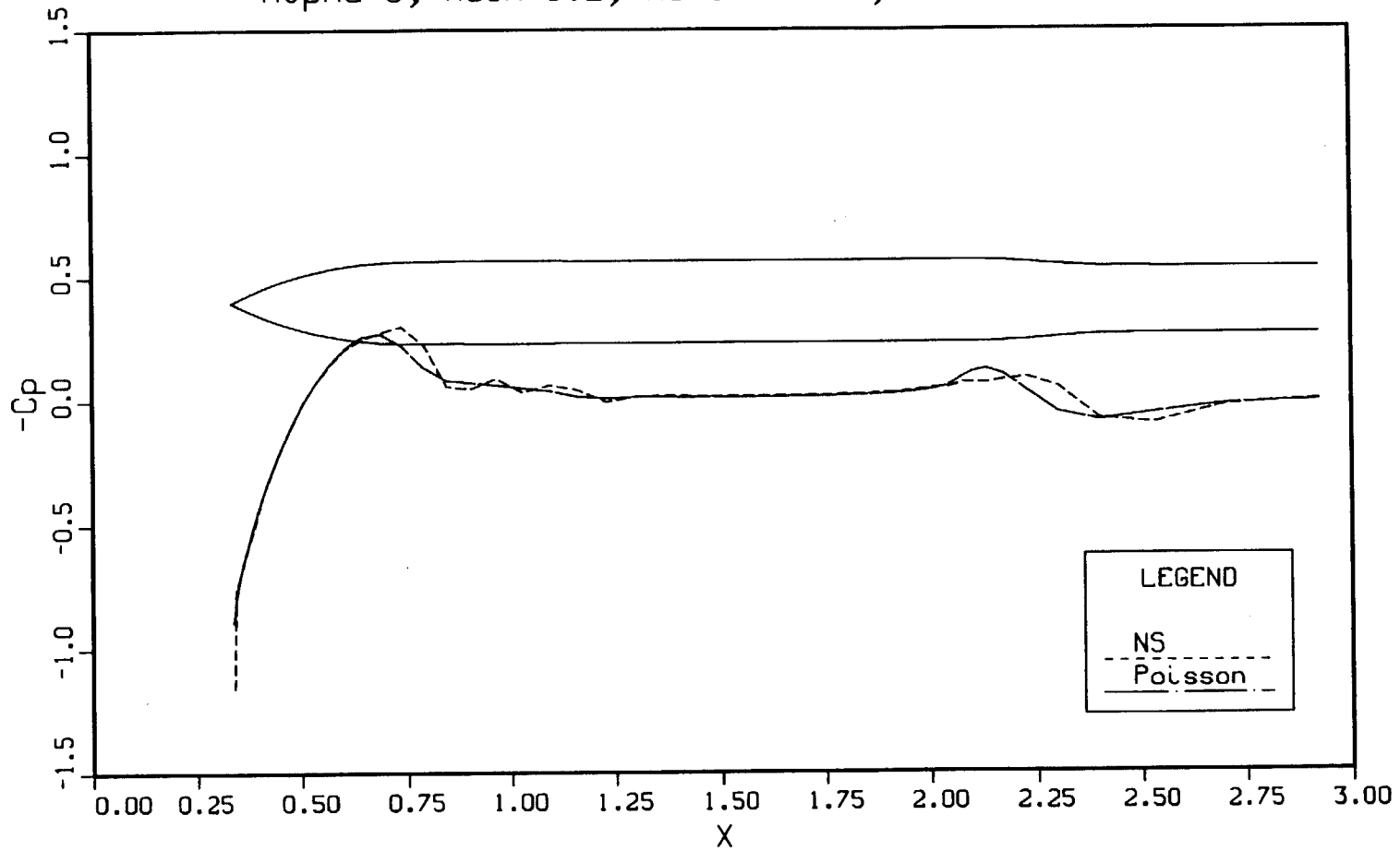
Figure 4.24: Comparison of surface pressure coefficients for the external tank, M_\infty = 0.2 , Re = 4.0 \times 10^6/ft , and \alpha = 0^\circ ( x in 10^3 inches)
