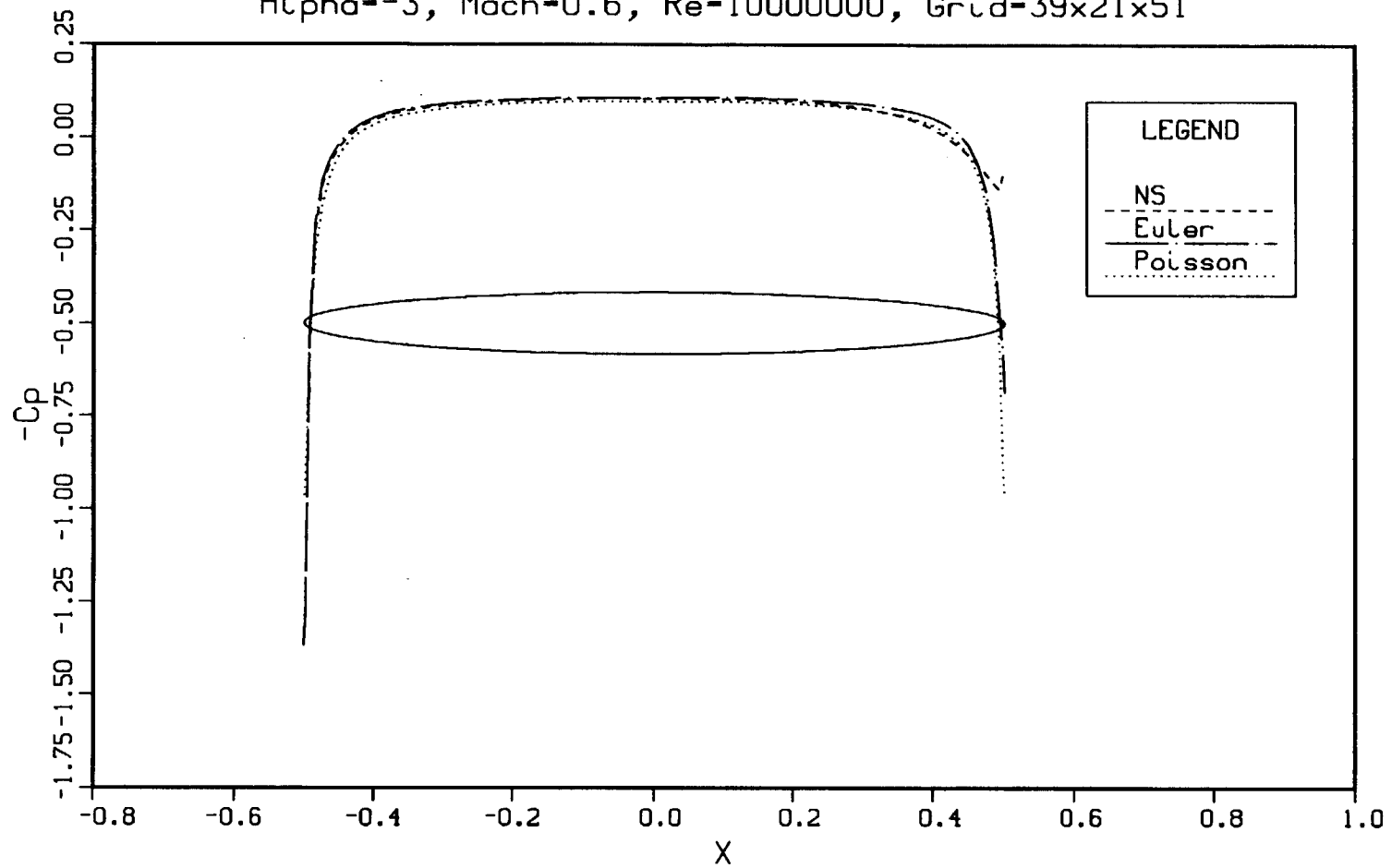
Figure 4.18: Comparison of C_p from the Poisson, Euler and Navier-Stokes solutions at the \phi = 90^\circ plane for an ellipsoid at M_\infty = 0.6 , Re = 10^7 , and \alpha = -3^\circ
