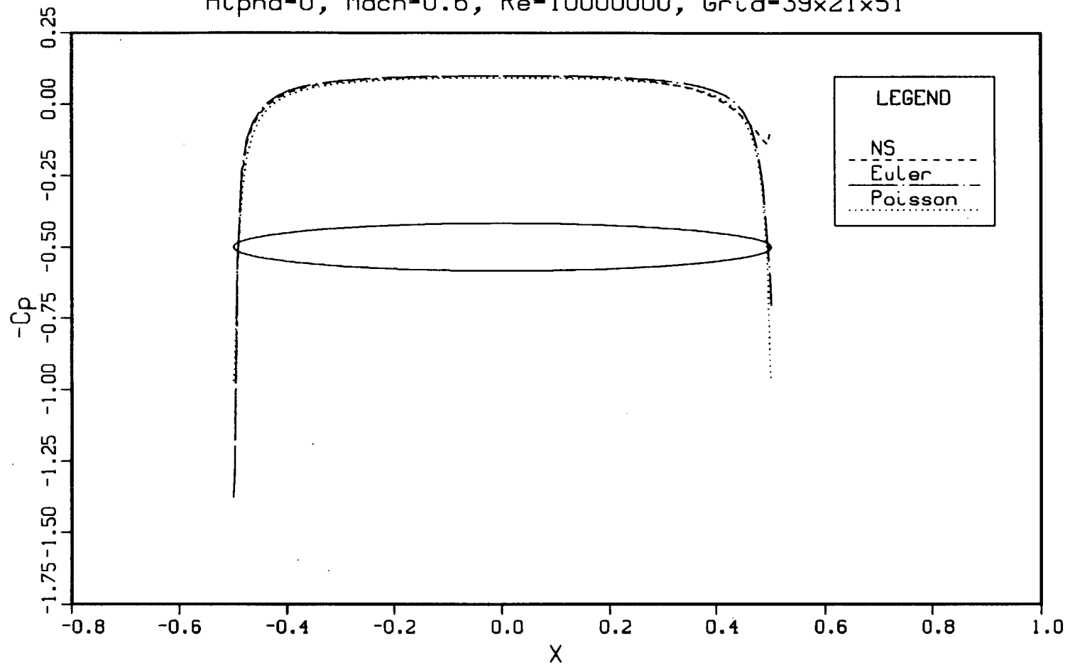
Figure 4.16: Comparison of C_p from the Poisson, Euler and Navier-Stokes solutions at the \phi = 90^\circ plane for an ellipsoid at M_\infty = 0.6 , Re = 10^7 , and \alpha = 0^\circ
