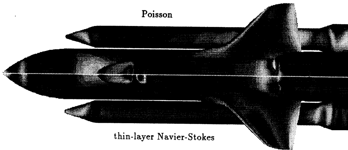
Figure 4.30: Comparison of C_p from the Poisson and thin-layer Navier-Stokes solutions for ISSV at M_\infty = 0.6 , Re = 4 \times 10^6/ft , and \alpha = -3^\circ
