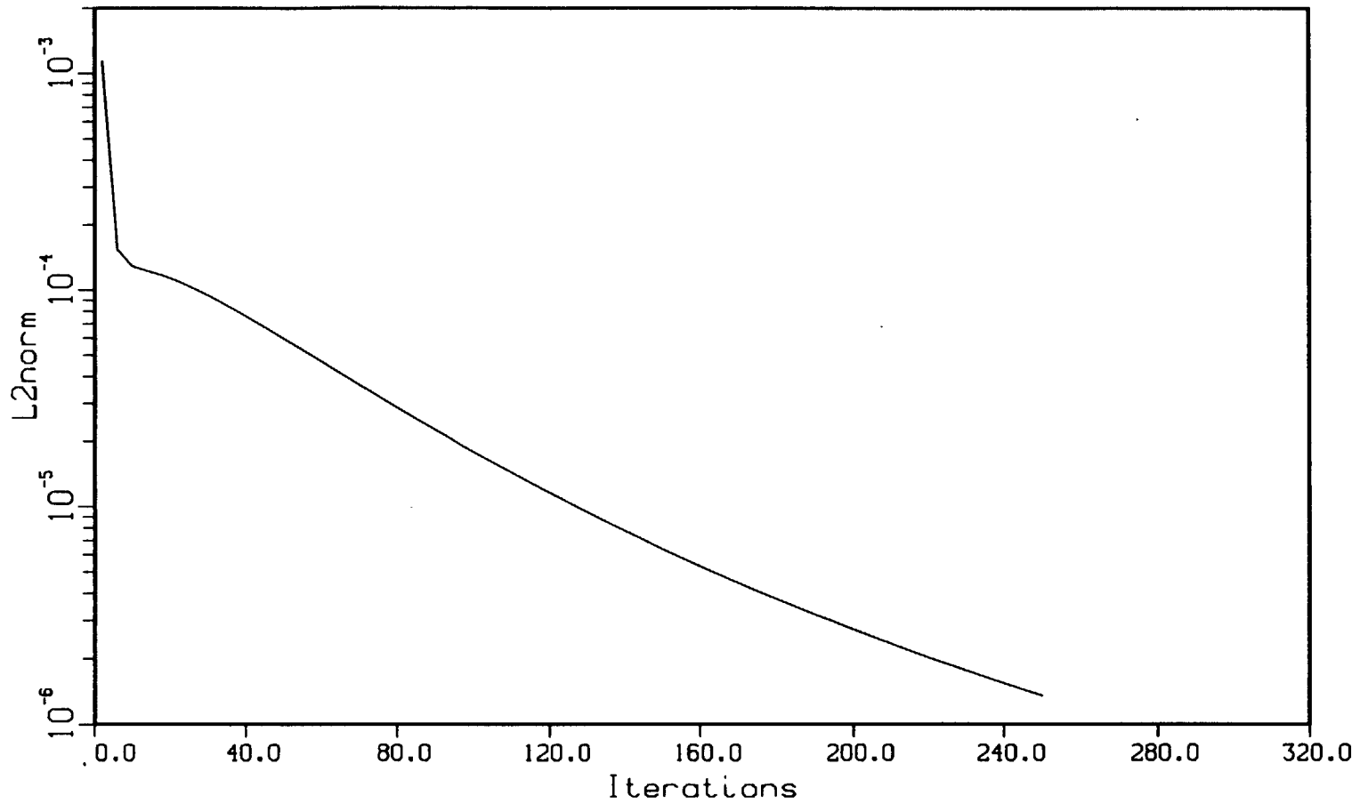
Figure 4.12: Convergence history of the Poisson solution for a sphere at M_{\infty} = 0.57 , and \alpha = 0^{\circ}
