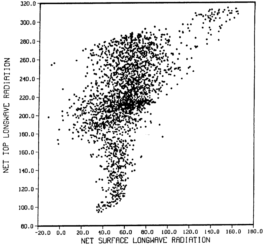
Figure 1. Monthly mean (July) outgoing longwave radiation at the top of the atmosphere plotted versus the net surface longwave radiation for each 4° lat x 5° long grid point of a general circulation model.
