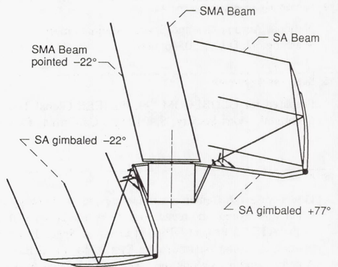
Figure 7.—ATDRS phased array and offset fed reflector configuration concept.
