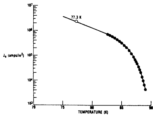
(c) CRITICAL CURRENT DENSITY OF YBa_2Cu_3O_7 ON SrTiO_3 .
