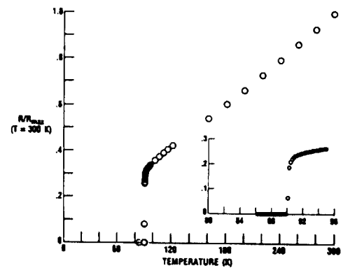
(b) RESISTANCE VERSUS TEMPERATURE OF YBa_2Cu_3O_7 .
