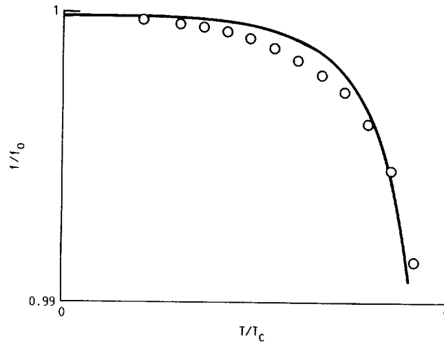
FIGURE 7. - RATIO OF THE OBSERVED RESONANT FREQUENCY ( f ) TO THE ZERO TEMPERATURE FREQUENCY ( f_0 ) VERSUS THE T/T_c . \circ 's REPRESENT EXPERIMENTAL VALUES. SOLID LINES REPRESENT CALCULATIONS BASED ON GORTER-CASIMIR MODEL.
