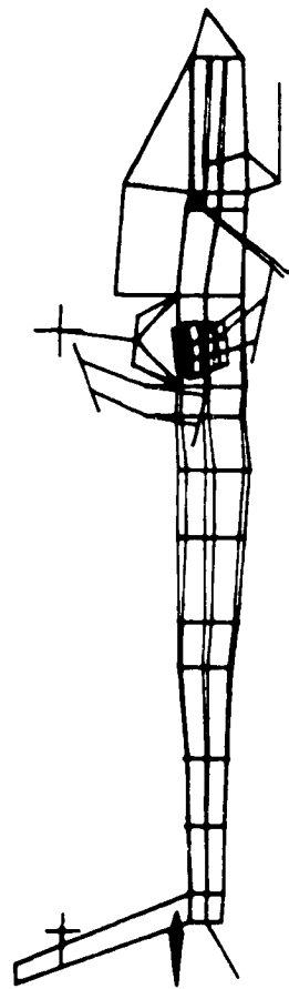
'LATERAL BENDING OF THE M/R MAST'
