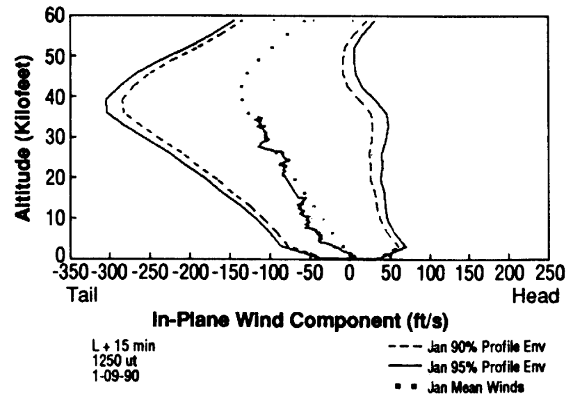
Figure 8. STS-32 prelaunch/launch Jimsphere-measured in-plane component winds (FPS). Flight azimuth = 90 degrees.
