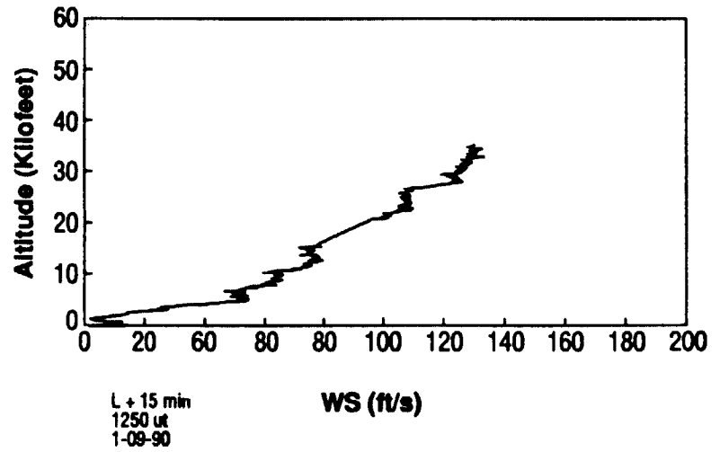
Figure 6. STS-32 prelaunch/launch Jimsphere-measured wind speeds (FPS).
