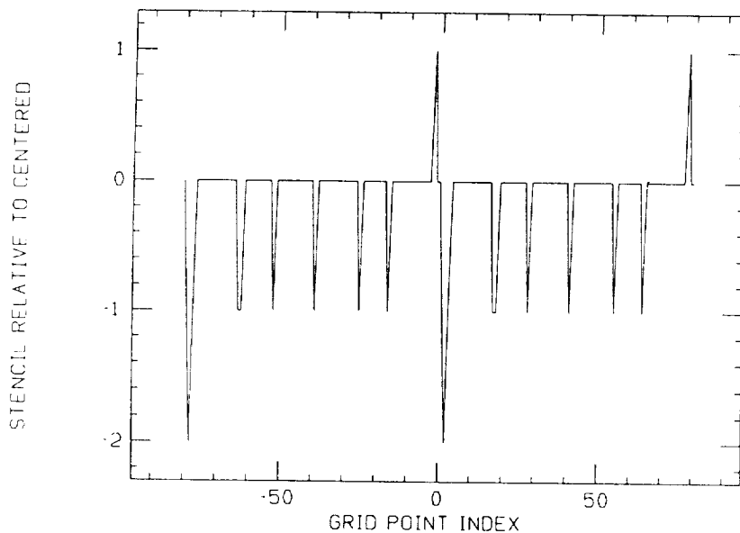
Figure 2f: same as 2b except that the modified ENO is used
