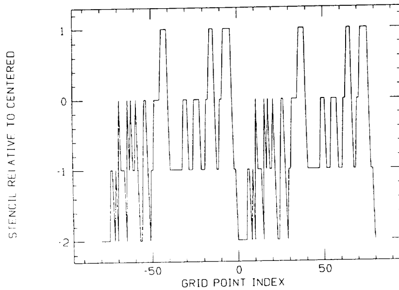
Figure 2d: same as 2b except that t = 4
