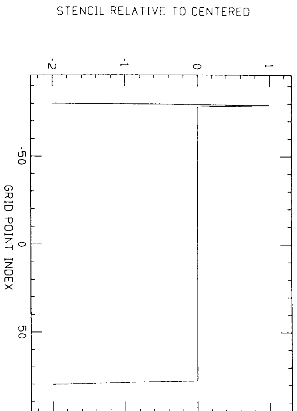
Figure 3h: same as 3b except that a modified ENO is used
