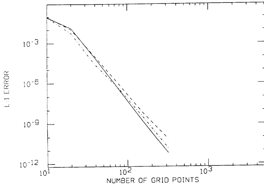
Figure 4c: same as 4a except that seventh order in space is used
