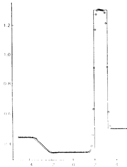
Figure 6b: same as 6a except that Circles: modified ENO
