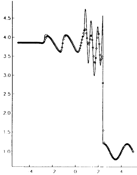
Figure 7a: shock interaction with density perturbations. (\rho_L, u_L, p_L) = (3.857143, 2.629369, 10.333333) , (\rho_R, u_R, p_R) = (1 + 0.2 \sin(5x), 0, 1) . Density is plotted. Solid line: a converged solution computed by ENO with 1200 grid points; Circles: ENO with 160 grid points
