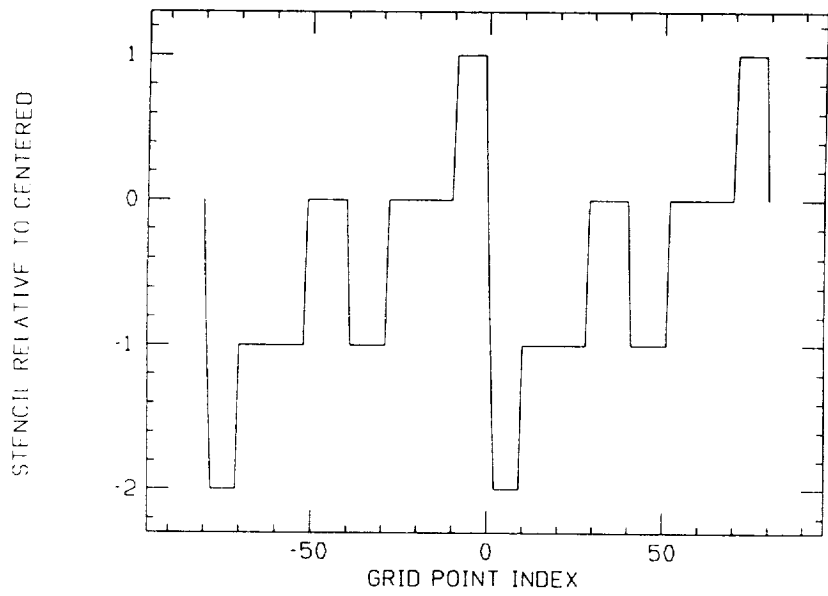
Figure 2b: same as 1b except that u^0(x) = \sin^4(\pi x)
