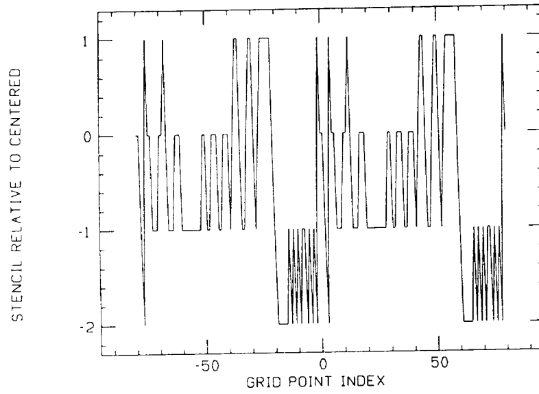
Figure 2c: same as 2b except that t = 100\Delta t
