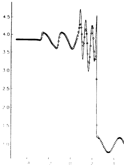
Figure 7b: same as 7a except that Circles: modified ENO with 160 grid points
