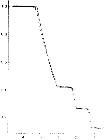
Figure 5b: same as 5a except that Circles: modified ENO
