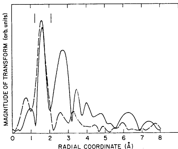
Fig. 4. The Fourier transforms of L_3 edge k^2\chi(k) for Au_2O_3 (dashed curve) and YBa_2Au_{0.3}Cu_{2.7}O_{7.6} (solid curve).
