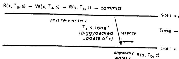
Fig. 4. Reduction in latency using piggybacked update.
