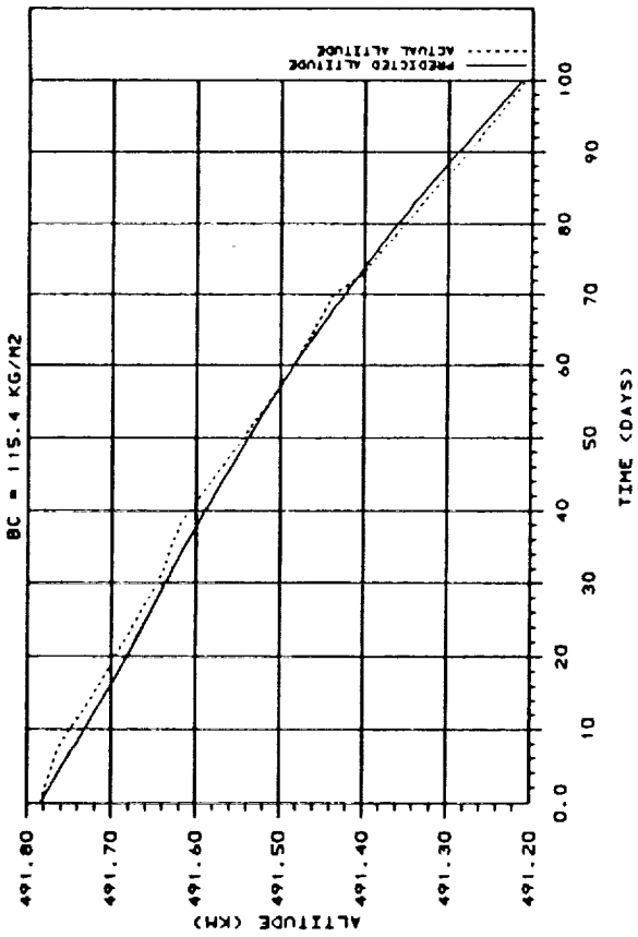
Figure 5. July 1986 ballistic coefficient calibration SMM.
