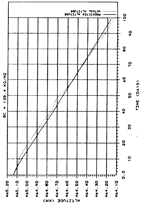
Figure 7. July 1986 ballistic coefficient calibration BP.
