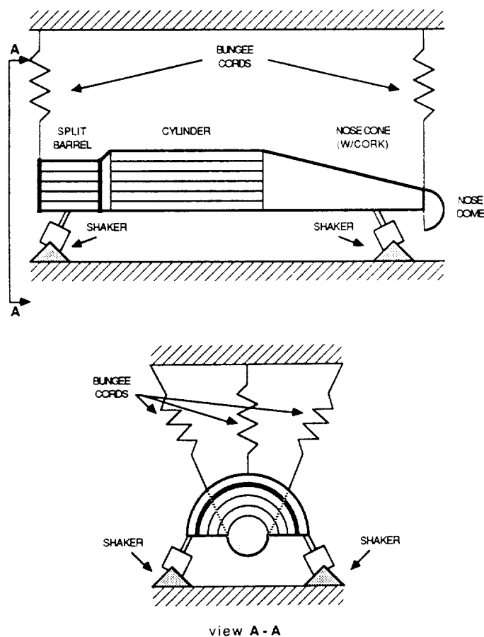
Figure 5. 11-Foot Diameter Payload Fairing Modal Test Free-Free Condition.
