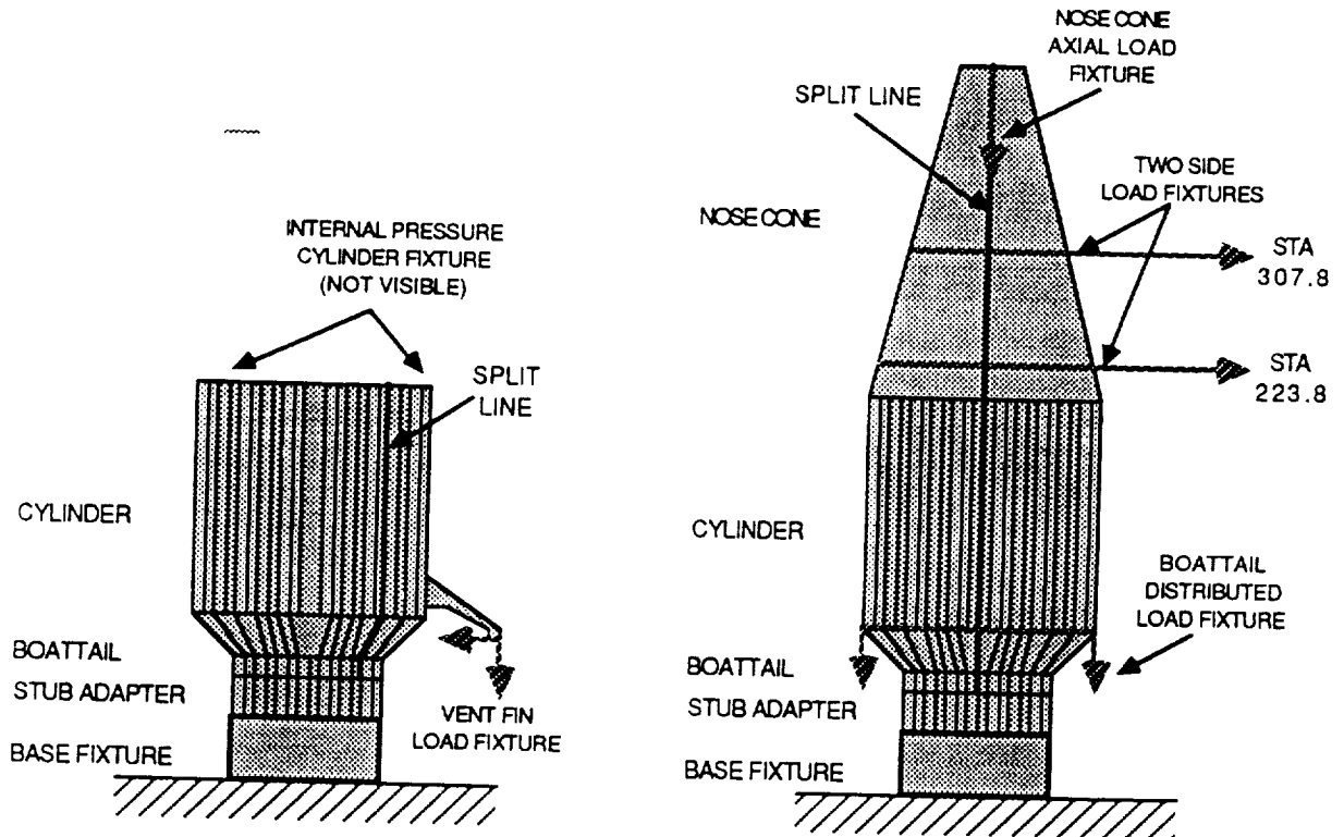
Figure 3c. Cylinder Burst Tests.
