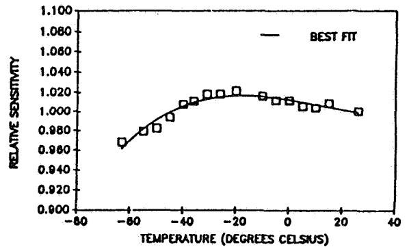
PYRGEOMETER #12150F3
