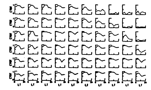
Figure 5. Diurnal variability of total cloud amount (%).
