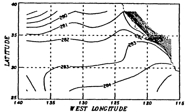
Figure 3. Mean cloud-top temperatures for July 1987.
