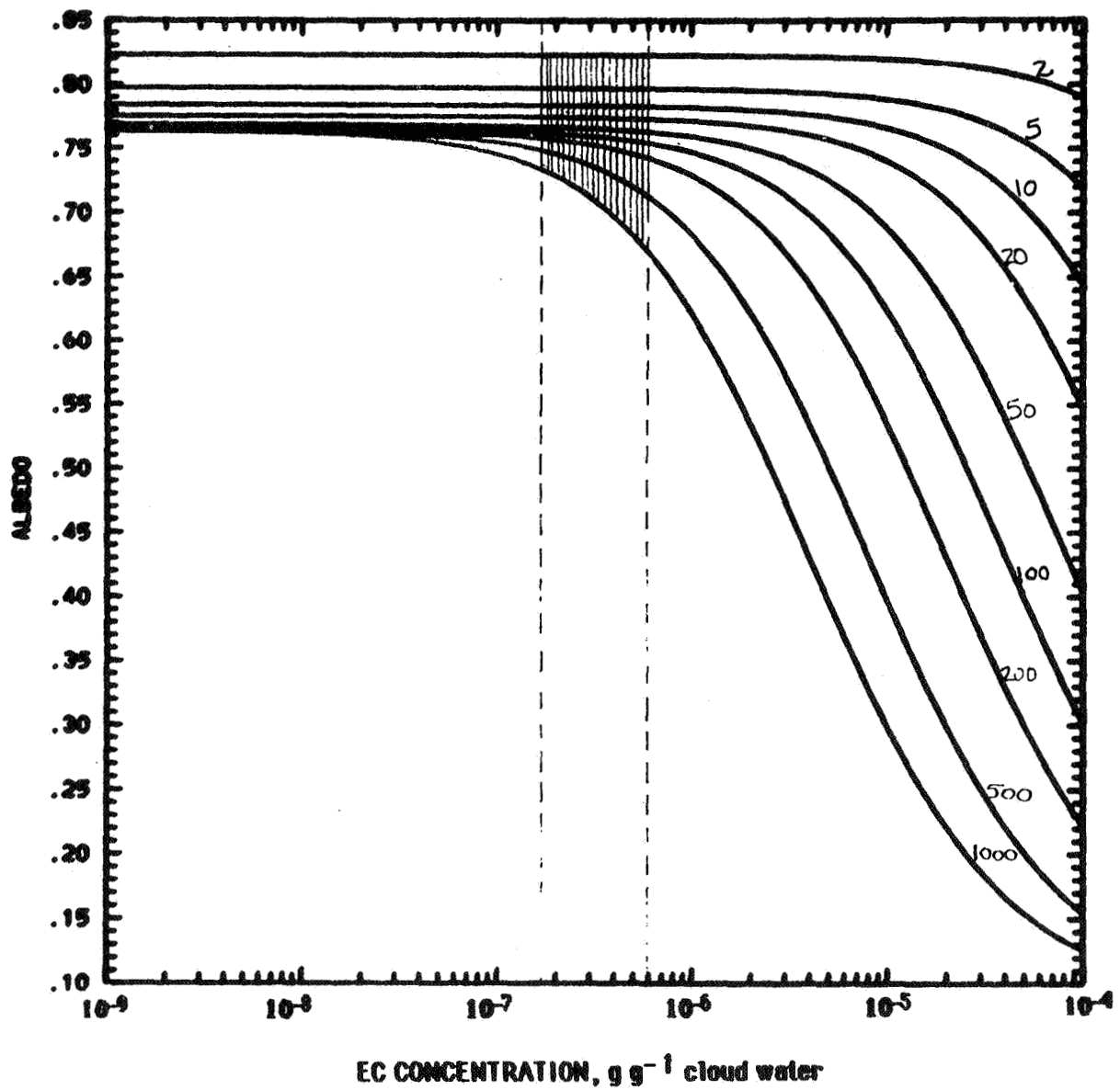
Figure 2. Same as Figure 1 except with a more realistic optical thickness of 30.
