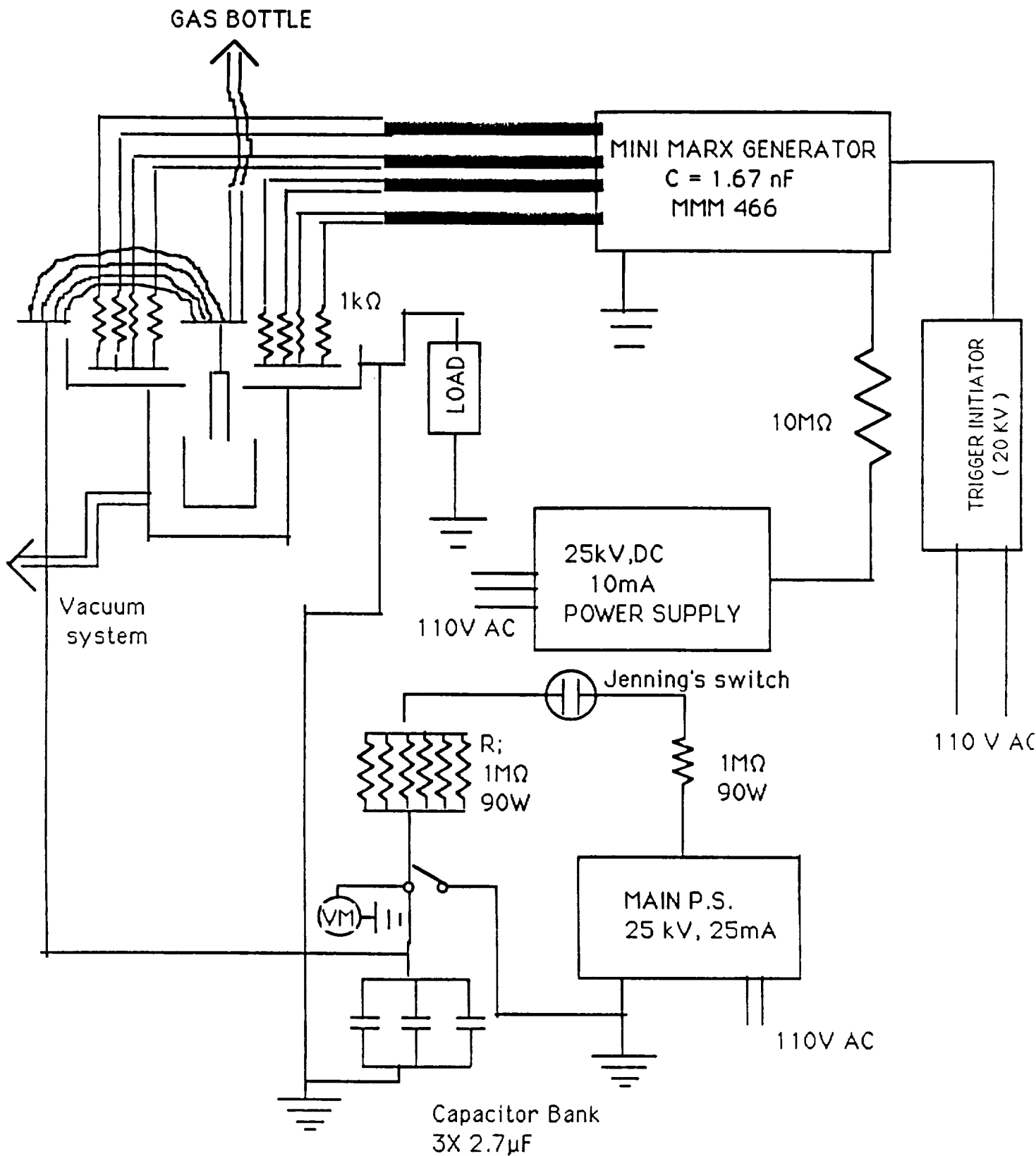
Figure 1. Schematic diagram of the plasma-puff triggering experiment based on the hypocycoloidal pinch geometry.
