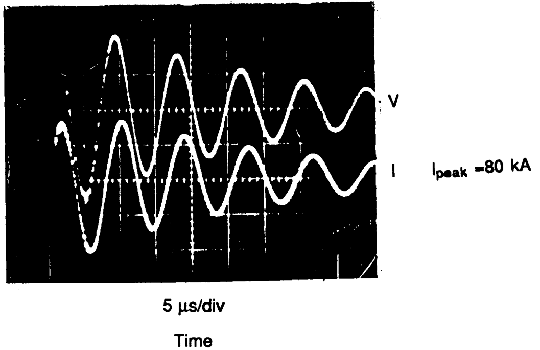
Figure 11. Voltage (upper) and current (lower) waveforms of inversepinch switch versus time. These data were obtained for a N 2 gas of 300 Torr under charging voltage of 13.5 kV to inner electrode of inverse pinch switch.
