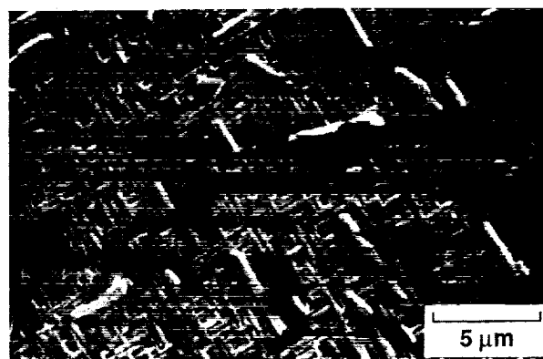
Figure 4. SEM micrograph of a 3000 Å thick co-sputtered post-annealed YBCO film on \text{LaAlO}_3 . The 'basket weave' structure is composed of YBCO grains with either the 'a' or 'b' axis normal to the substrate.
