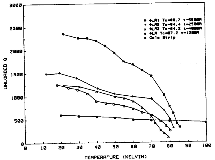
Figure 5. Unloaded Q vs temperature for several laser ablated films on LaAlO 3 . All films eventually perform better than the gold implementation of the resonator. The best film is four times better at 20°K than the gold resonator.
