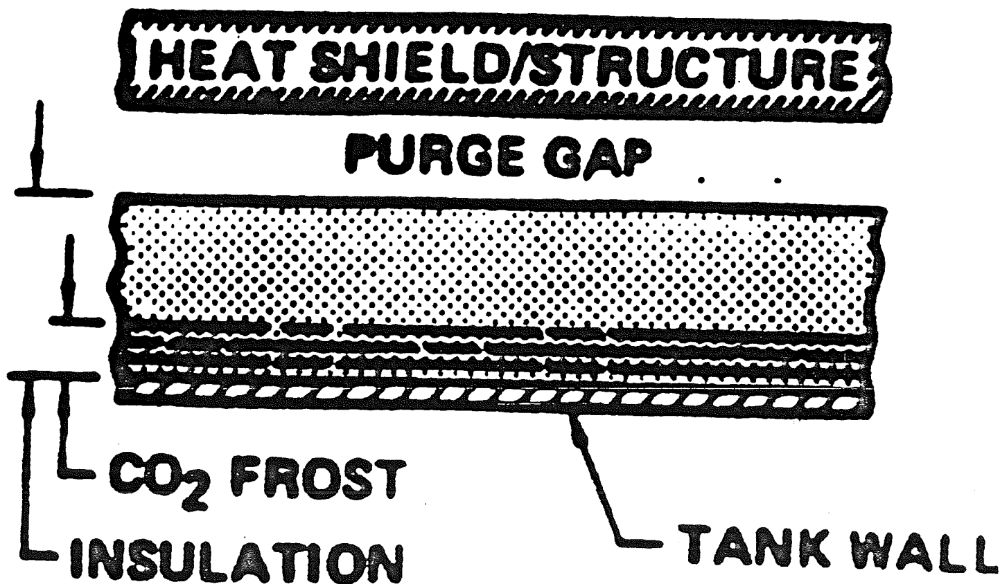
Figure MS7: CO 2 purge System
