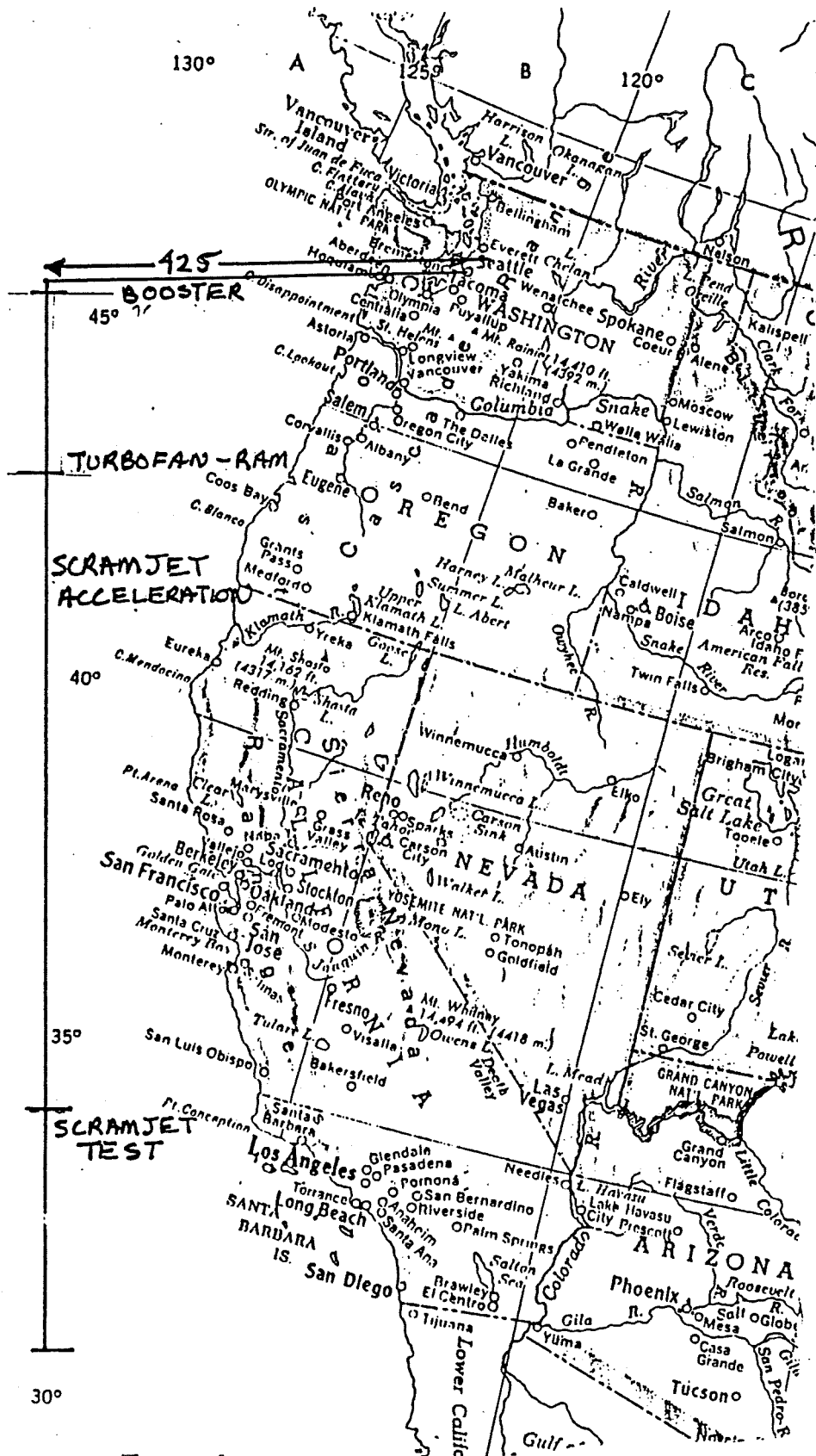
FIG. PROFILE 2 FLIGHT PATH
