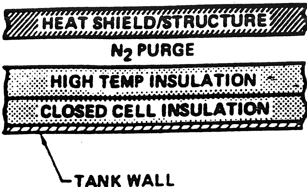
Figure MS6: N 2 purge System
