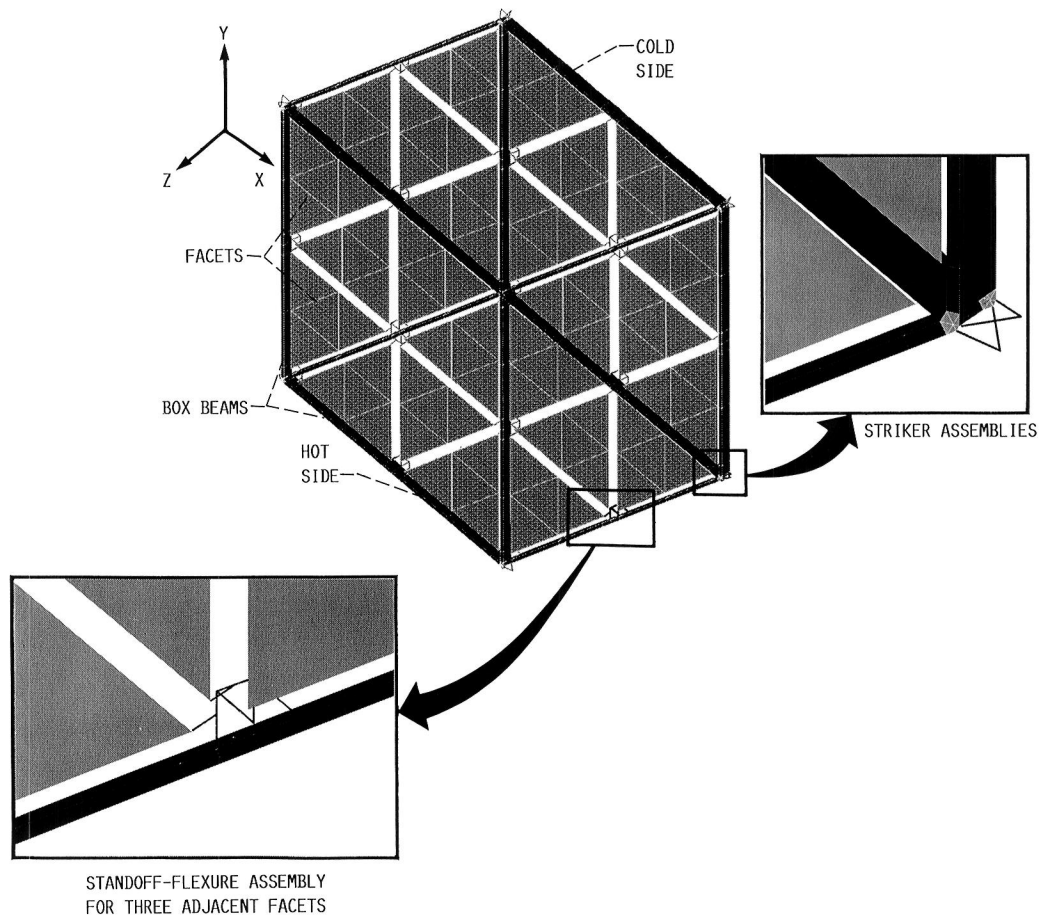
FIGURE 8. - HEXPANEL FINITE ELEMENT MODEL.
