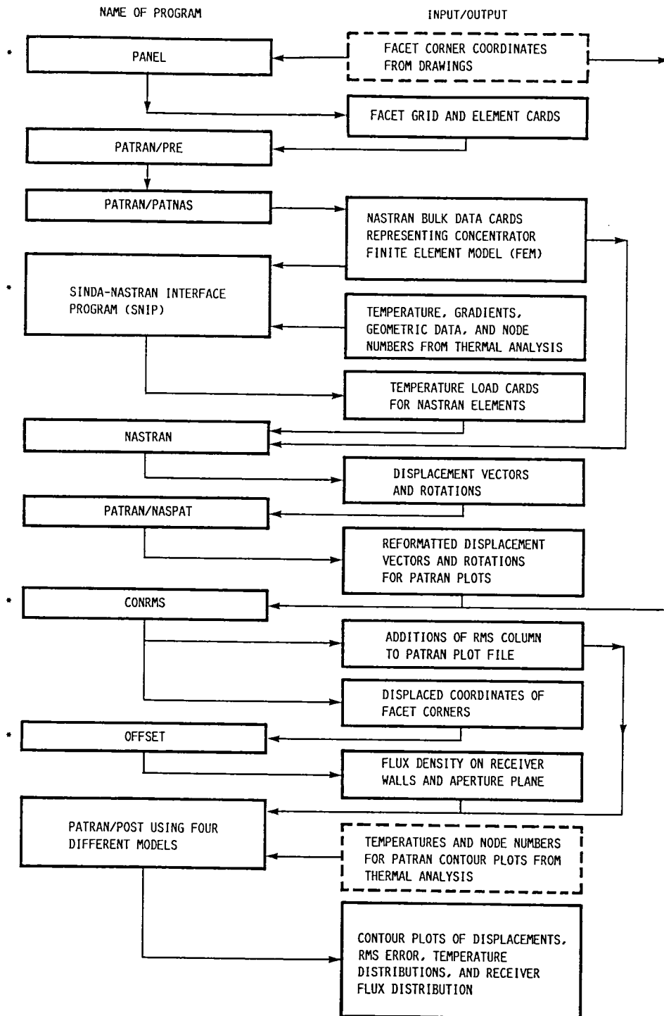
FIGURE 11. - CONCENTRATOR THERMAL DISTORTION ANALYSIS PROCEDURE. (ASTERISK DENOTES PROGRAMS DEVELOPED AT LEWIS RESEARCH CENTER.)
