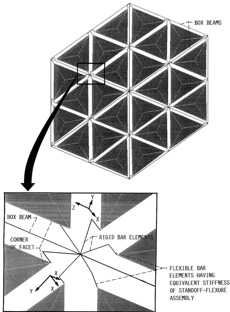
FIGURE 9. - CONCENTRATOR FINITE ELEMENT MODEL - SINGLE HEXPANEL.
