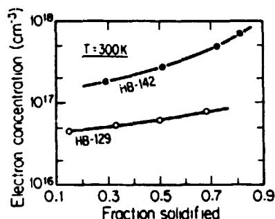
FIG. 5. Free-electron concentration in GaAs crystal HB-142 grown with V powder outside the boat in the growth ampule. Crystal HB-129 is V free.
