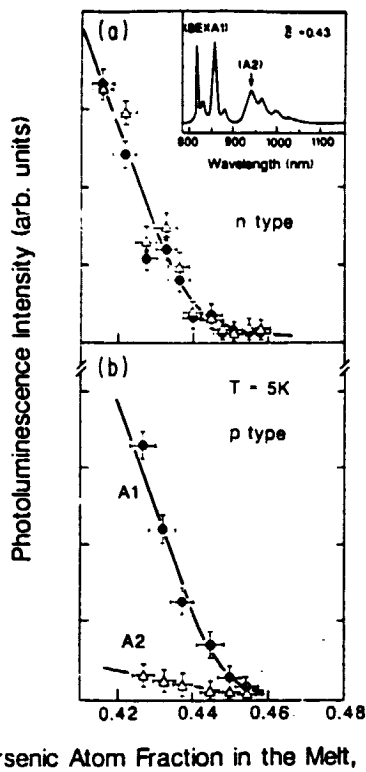
FIG. 1. Stoichiometry dependence of the intensity of characteristic PL lines: A1 at 1.443 eV and A2 at 1.320 eV in (a) n -type and (b) p -type crystals. Insert in (a) shows the typical low-temperature PL spectrum. The free-carrier concentration for all the samples was of the order of 10^{16} \text{ cm}^{-3} .
