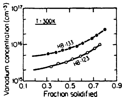
FIG. 3. Concentration of V acceptors along two HB V-doped crystals determined by the optical method described in Ref. 11. The effective segregation coefficient of V in GaAs determined from these curves is about 5.2 \times 10^{-3} .
