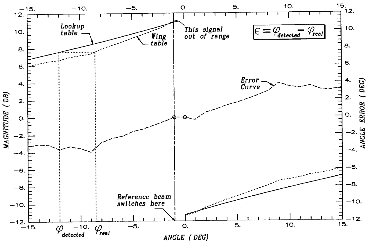
Figure 3.10: Calculation of bearing error.
